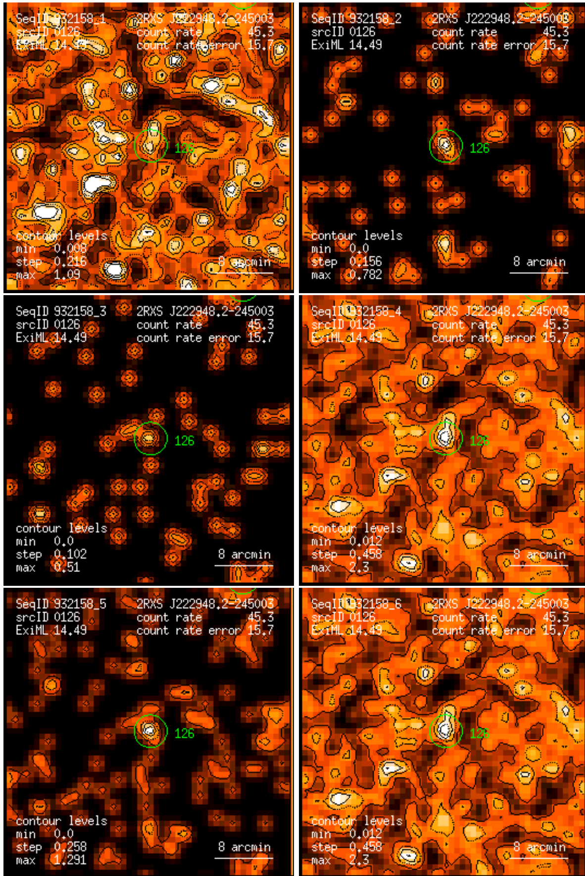
Figure 126: RASS 932158: detection 0126: band rate images, Gaussian filter: (1) PSPC channels 11 – 41, (2) 52 – 90, (3) 91 – 201, (4) 11 – 235, (5) 52 – 201, (6) 11 – 201. Broad band rates in counts/ks. Band rate contour levels in counts/ks/arcmin 2 .
