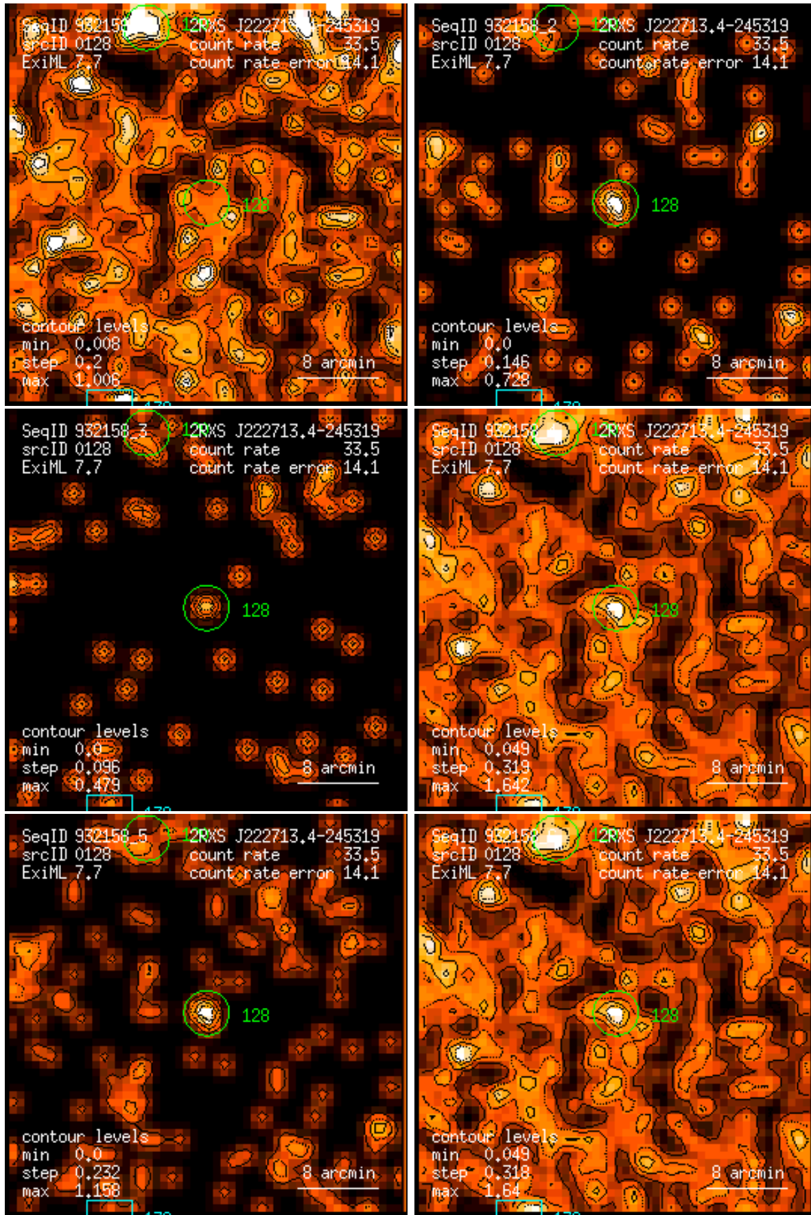
Figure 128: RASS 932158: detection 0128: band rate images, Gaussian filter: (1) PSPC channels 11 – 41, (2) 52 – 90, (3) 91 – 201, (4) 11 – 235, (5) 52 – 201, (6) 11 – 201. Broad band rates in counts/ks. Band rate contour levels in counts/ks/arcmin 2 .
