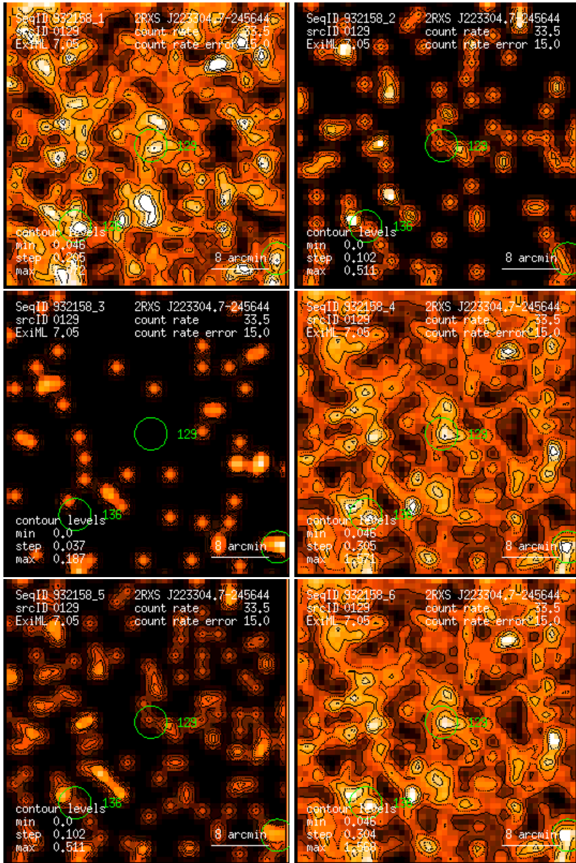
Figure 129: RASS 932158: detection 0129: band rate images, Gaussian filter: (1) PSPC channels 11 – 41, (2) 52 – 90, (3) 91 – 201, (4) 11 – 235, (5) 52 – 201, (6) 11 – 201. Broad band rates in counts/ks. Band rate contour levels in counts/ks/arcmin 2 .
