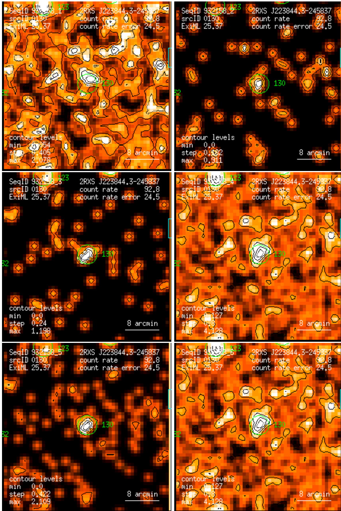
Figure 130: RASS 932158: detection 0130: band rate images, Gaussian filter: (1) PSPC channels 11 – 41, (2) 52 – 90, (3) 91 – 201, (4) 11 – 235, (5) 52 – 201, (6) 11 – 201. Broad band rates in counts/ks. Band rate contour levels in counts/ks/arcmin 2 .
