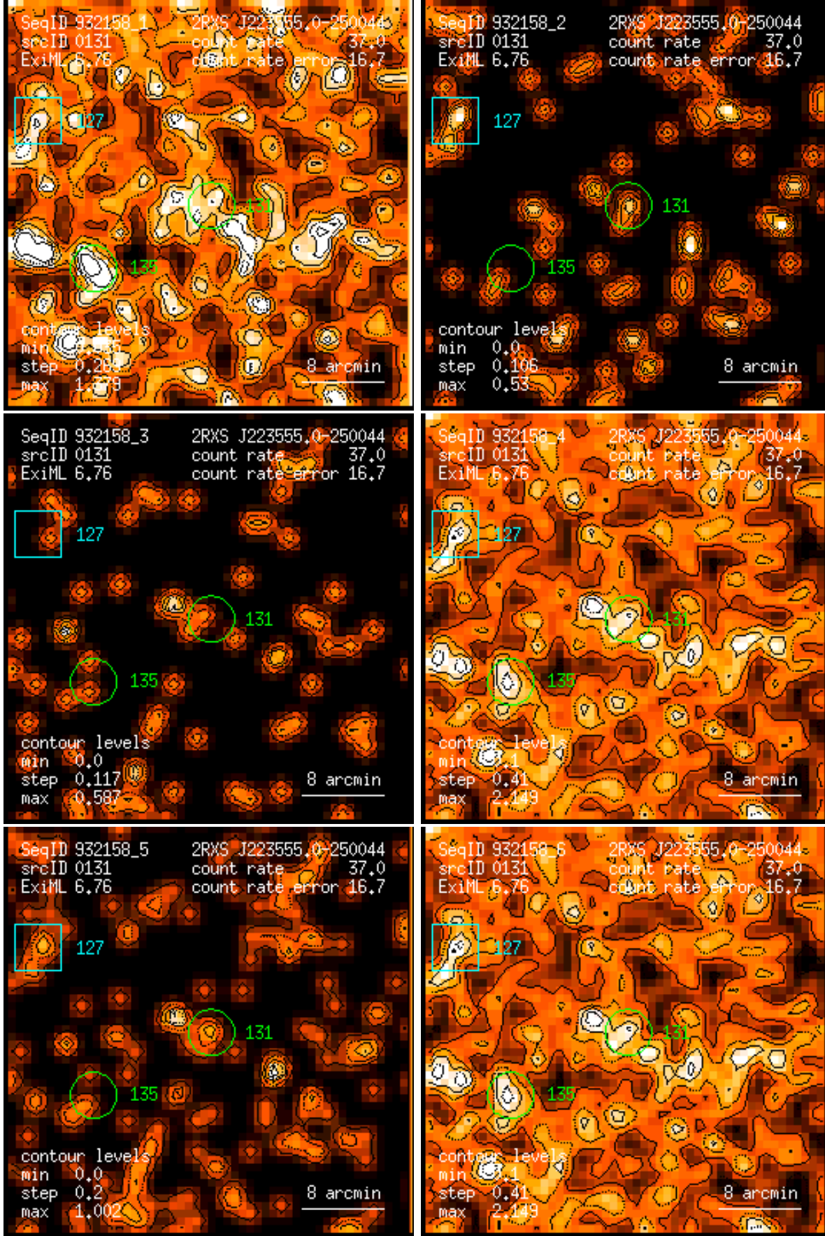
Figure 131: RASS 932158: detection 0131: band rate images, Gaussian filter: (1) PSPC channels 11 – 41, (2) 52 – 90, (3) 91 – 201, (4) 11 – 235, (5) 52 – 201, (6) 11 – 201. Broad band rates in counts/ks. Band rate contour levels in counts/ks/arcmin 2 .
