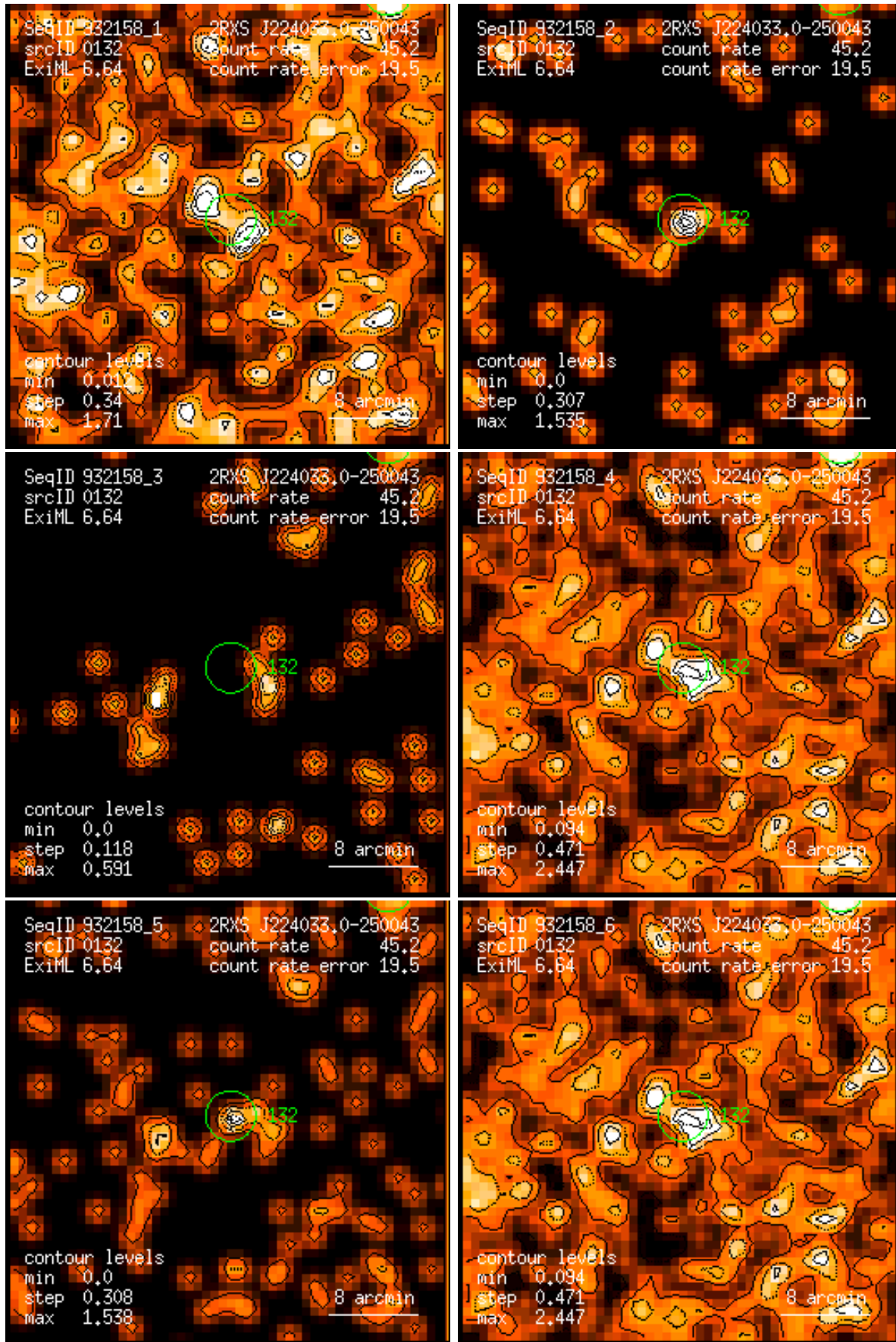
Figure 132: RASS 932158: detection 0132: band rate images, Gaussian filter: (1) PSPC channels 11 – 41, (2) 52 – 90, (3) 91 – 201, (4) 11 – 235, (5) 52 – 201, (6) 11 – 201. Broad band rates in counts/ks. Band rate contour levels in counts/ks/arcmin 2 .
