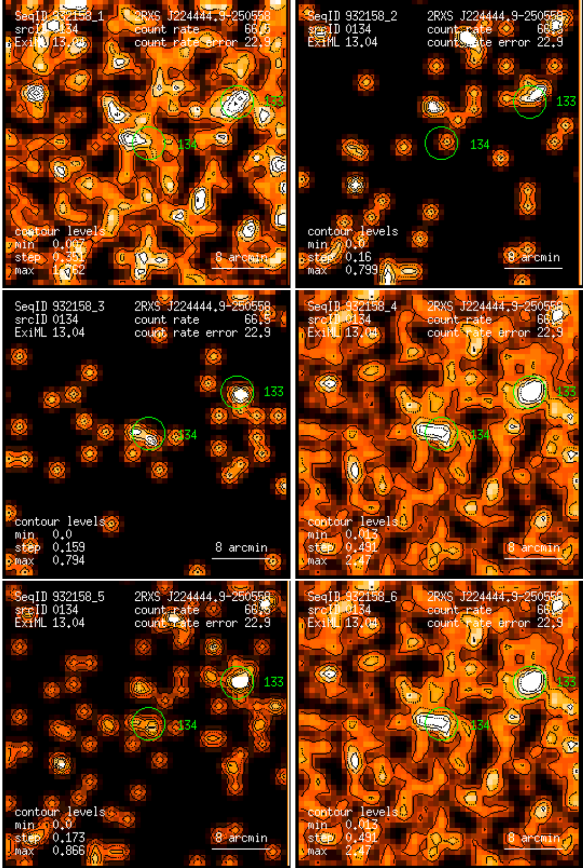
Figure 134: RASS 932158: detection 0134: band rate images, Gaussian filter: (1) PSPC channels 11 – 41, (2) 52 – 90, (3) 91 – 201, (4) 11 – 235, (5) 52 – 201, (6) 11 – 201. Broad band rates in counts/ks. Band rate contour levels in counts/ks/arcmin 2 .
