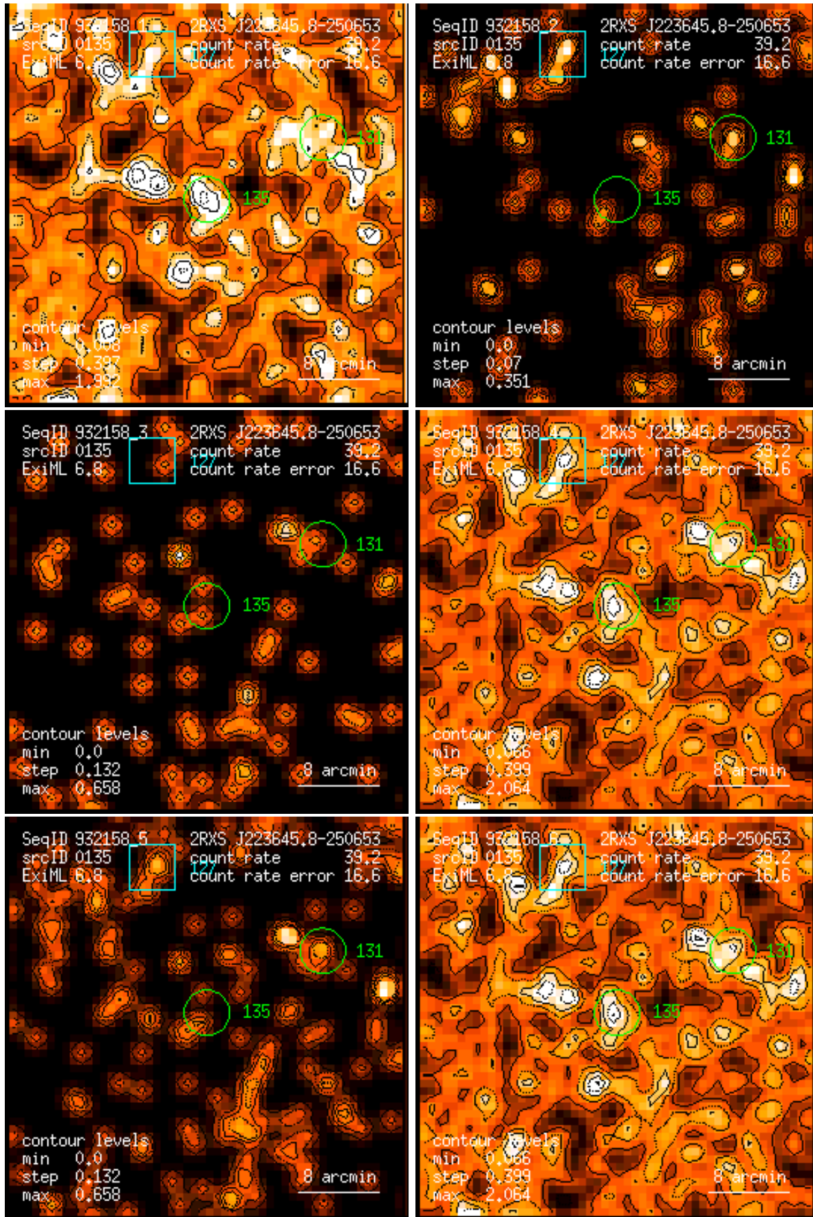
Figure 135: RASS 932158: detection 0135: band rate images, Gaussian filter: (1) PSPC channels 11 – 41, (2) 52 – 90, (3) 91 – 201, (4) 11 – 235, (5) 52 – 201, (6) 11 – 201. Broad band rates in counts/ks. Band rate contour levels in counts/ks/arcmin 2 .
