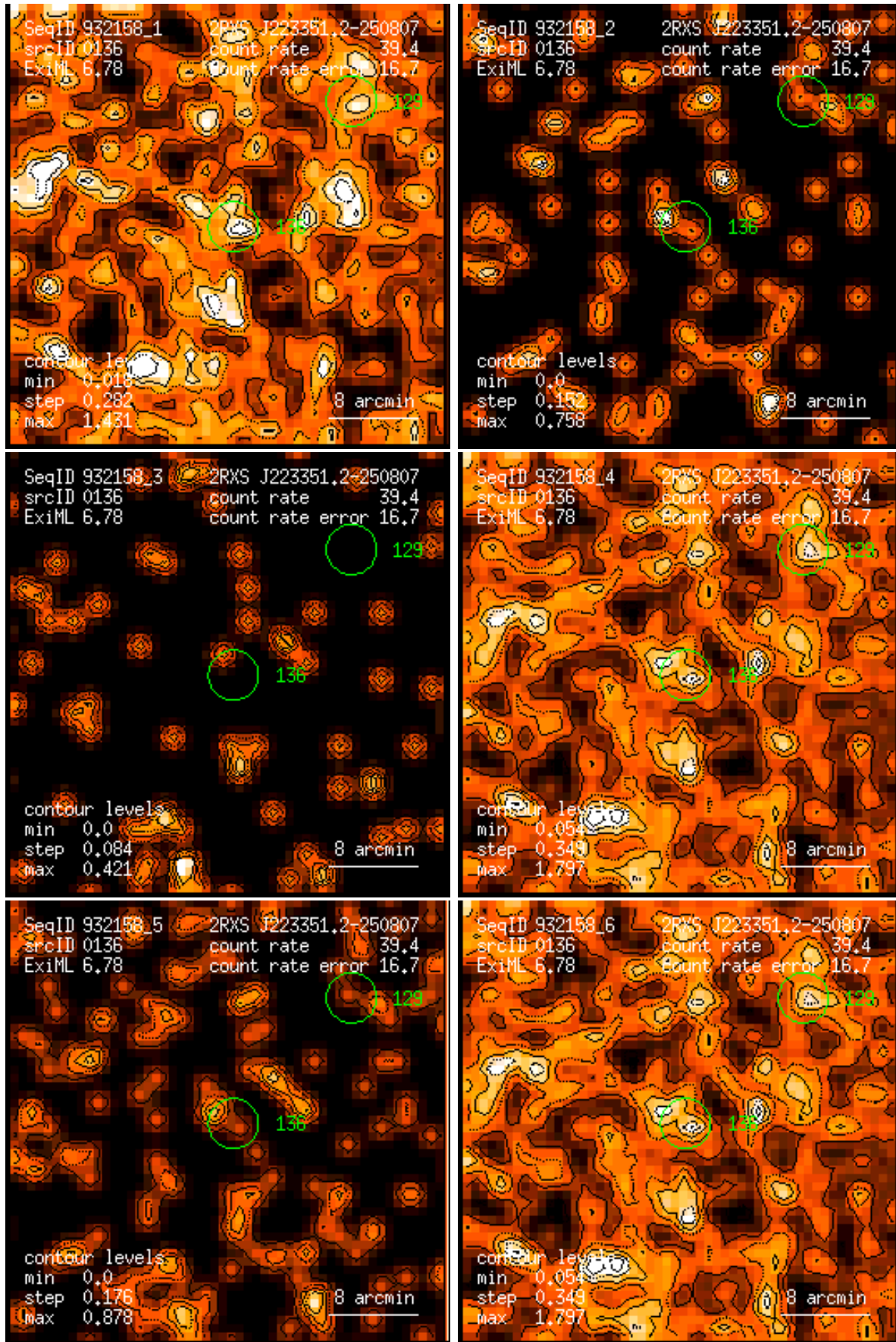
Figure 136: RASS 932158: detection 0136: band rate images, Gaussian filter: (1) PSPC channels 11 – 41, (2) 52 – 90, (3) 91 – 201, (4) 11 – 235, (5) 52 – 201, (6) 11 – 201. Broad band rates in counts/ks. Band rate contour levels in counts/ks/arcmin 2 .
