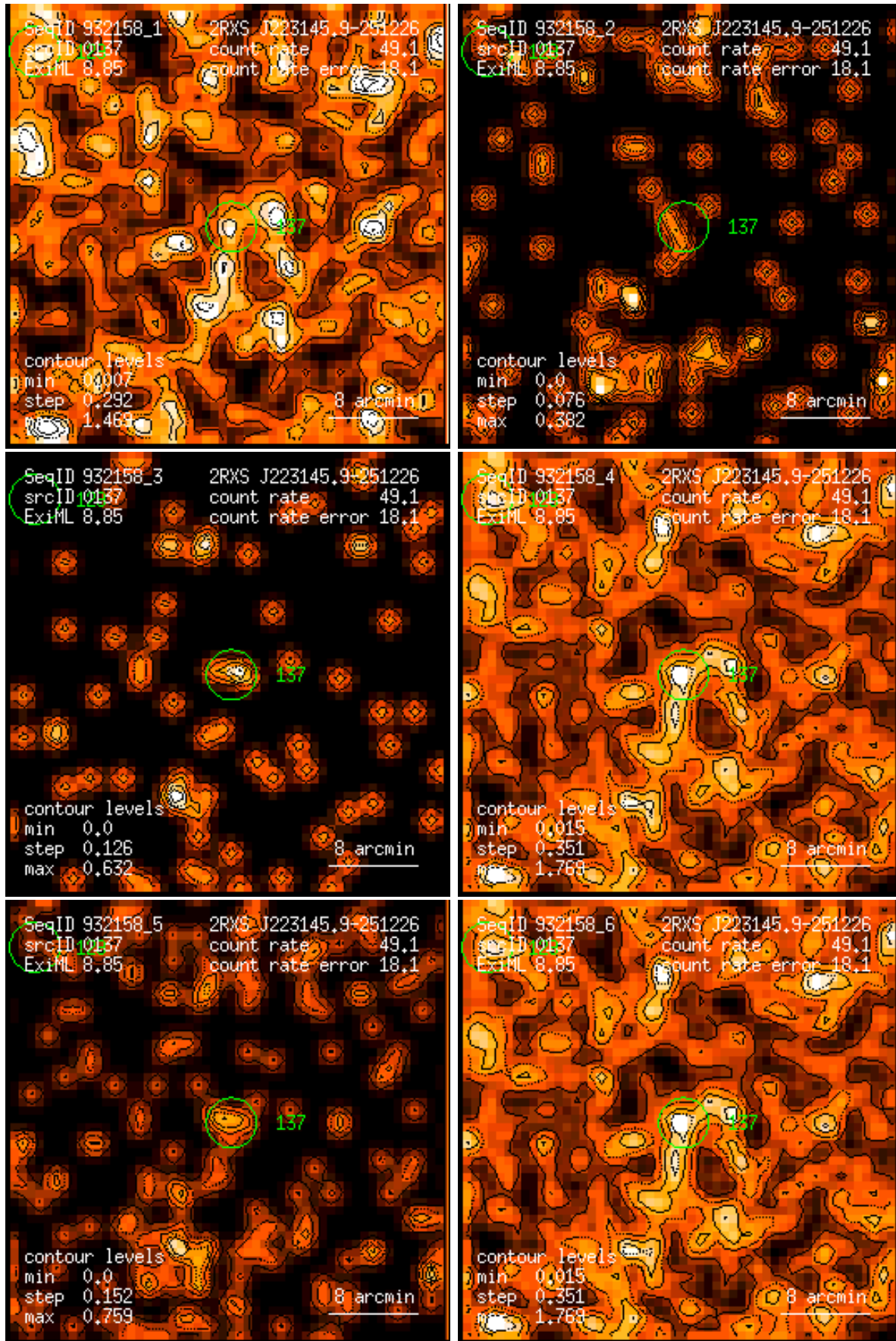
Figure 137: RASS 932158: detection 0137: band rate images, Gaussian filter: (1) PSPC channels 11 – 41, (2) 52 – 90, (3) 91 – 201, (4) 11 – 235, (5) 52 – 201, (6) 11 – 201. Broad band rates in counts/ks. Band rate contour levels in counts/ks/arcmin 2 .
