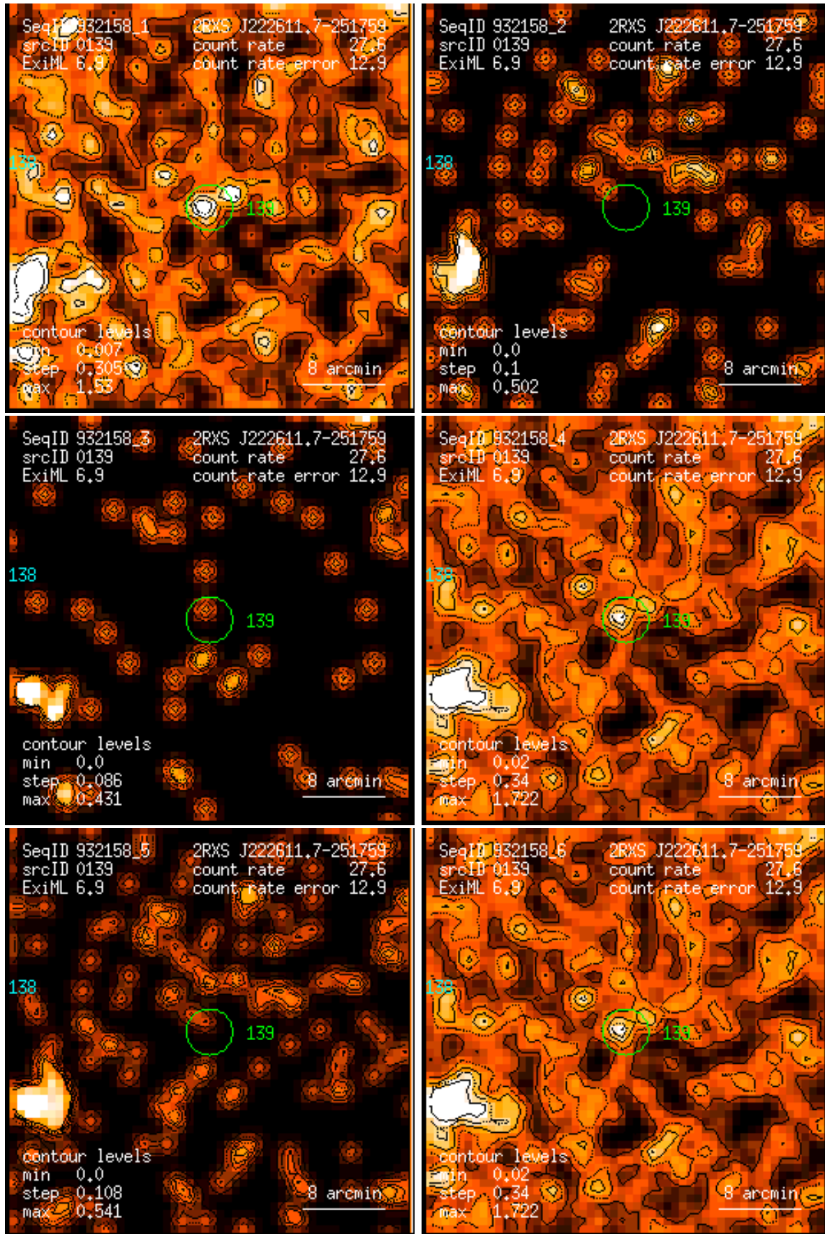
Figure 139: RASS 932158: detection 0139: band rate images, Gaussian filter: (1) PSPC channels 11 – 41, (2) 52 – 90, (3) 91 – 201, (4) 11 – 235, (5) 52 – 201, (6) 11 – 201. Broad band rates in counts/ks. Band rate contour levels in counts/ks/arcmin 2 .
