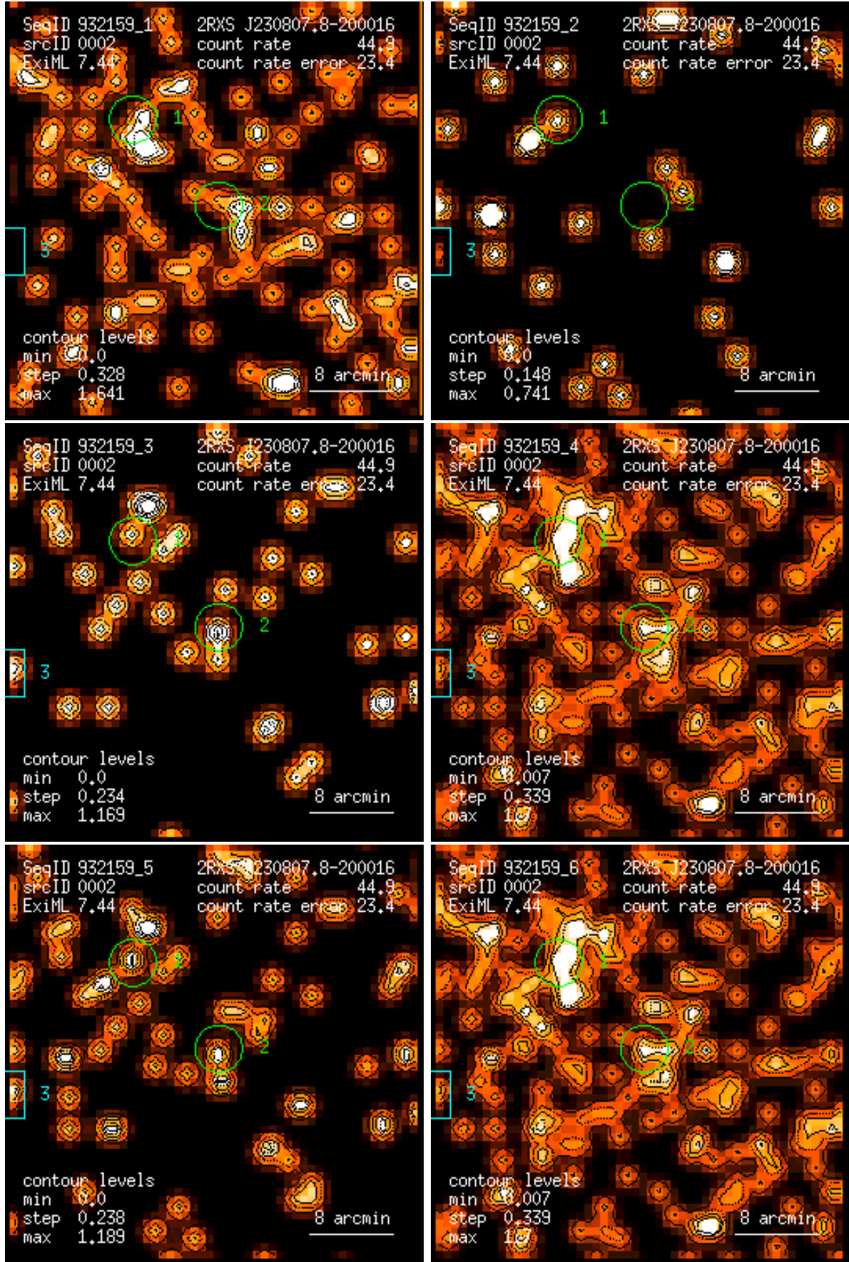
Figure 2: RASS 932159: detection 0002: band rate images, Gaussian filter: (1) PSPC channels 11 – 41, (2) 52 – 90, (3) 91 – 201, (4) 11 – 235, (5) 52 – 201, (6) 11 – 201. Broad band rates in counts/ks. Band rate contour levels in counts/ks/arcmin 2 .
