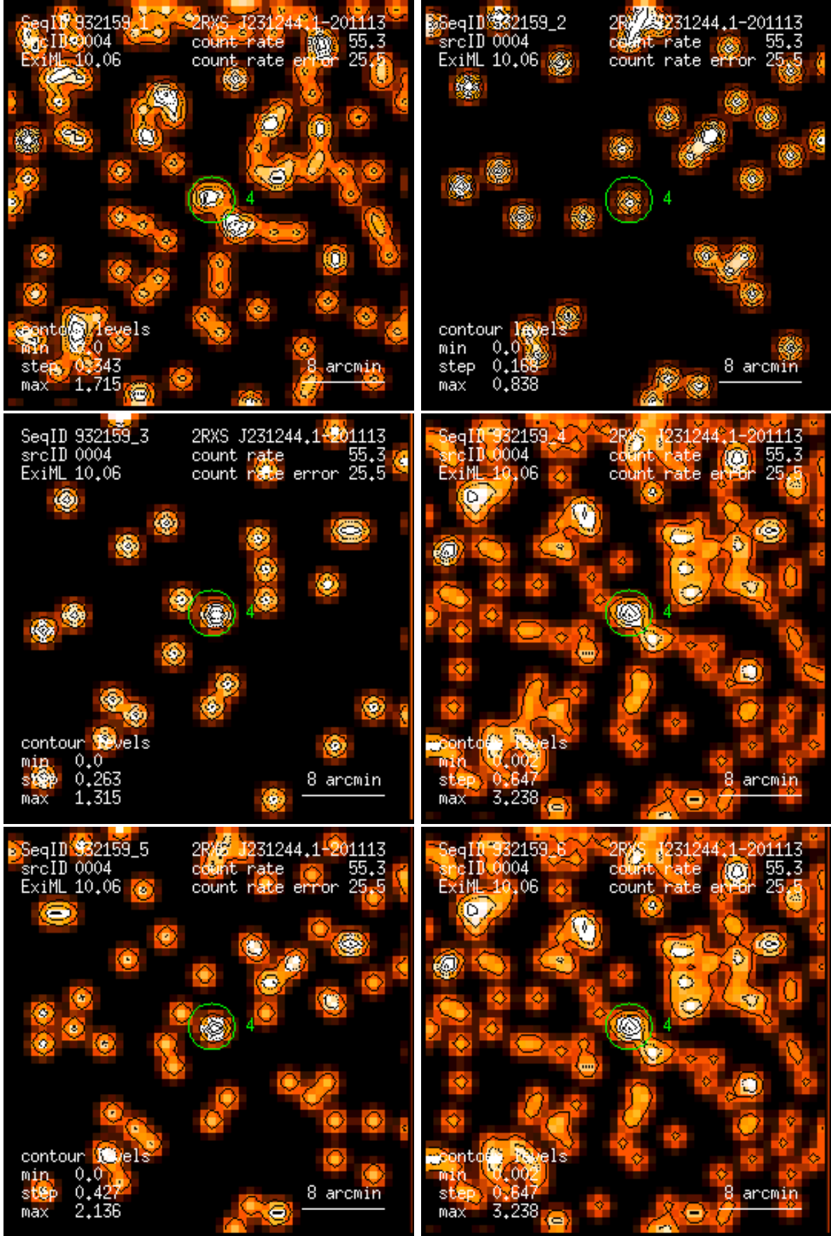
Figure 4: RASS 932159: detection 0004: band rate images, Gaussian filter: (1) PSPC channels 11 – 41, (2) 52 – 90, (3) 91 – 201, (4) 11 – 235, (5) 52 – 201, (6) 11 – 201. Broad band rates in counts/ks. Band rate contour levels in counts/ks/arcmin 2 .
