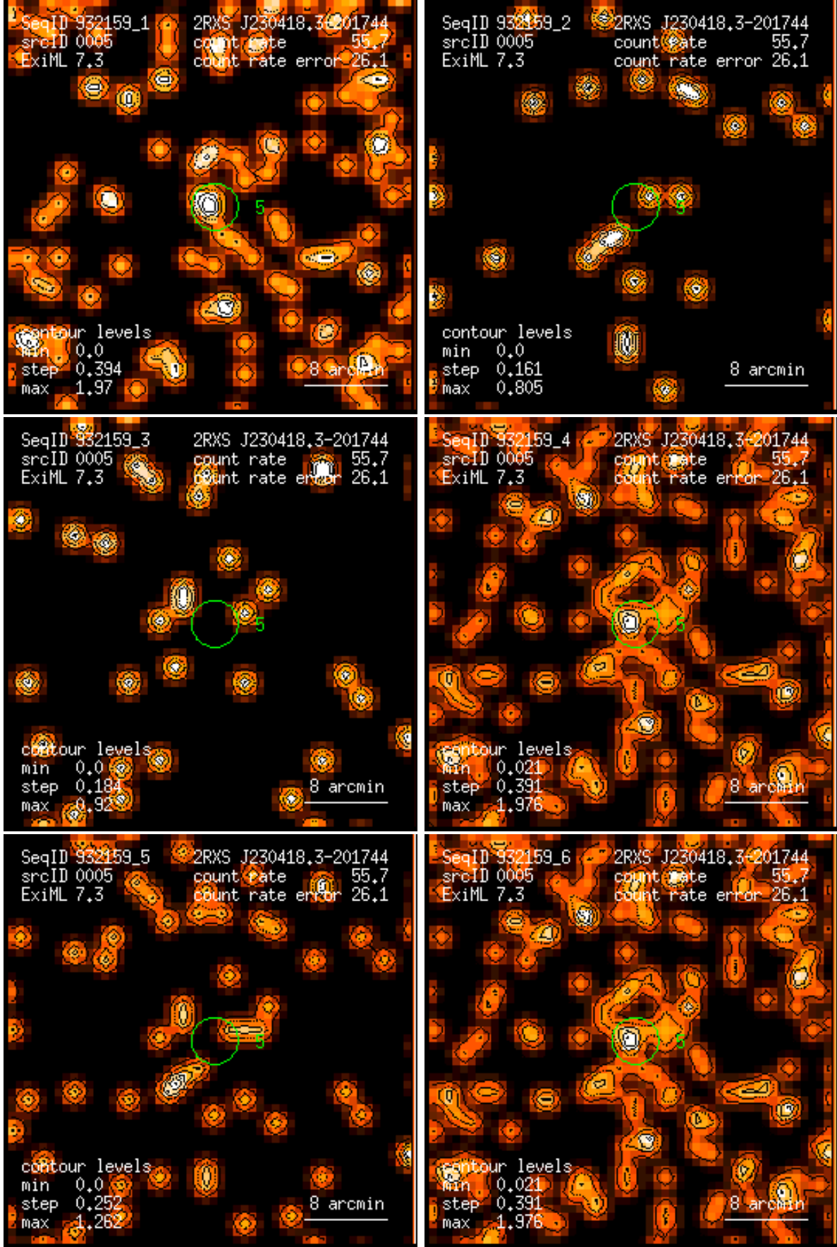
Figure 5: RASS 932159: detection 0005: band rate images, Gaussian filter: (1) PSPC channels 11 – 41, (2) 52 – 90, (3) 91 – 201, (4) 11 – 235, (5) 52 – 201, (6) 11 – 201. Broad band rates in counts/ks. Band rate contour levels in counts/ks/arcmin 2 .
