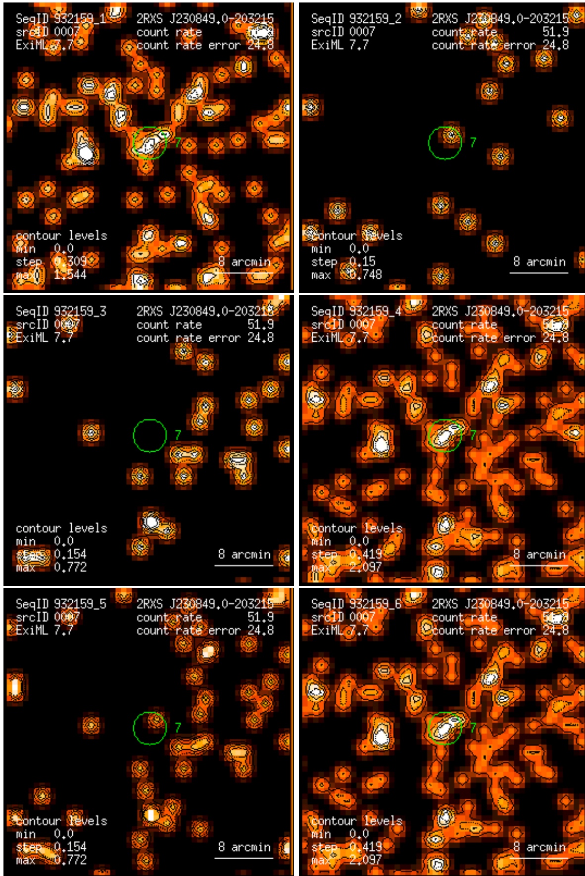
Figure 7: RASS 932159: detection 0007: band rate images, Gaussian filter: (1) PSPC channels 11 – 41, (2) 52 – 90, (3) 91 – 201, (4) 11 – 235, (5) 52 – 201, (6) 11 – 201. Broad band rates in counts/ks. Band rate contour levels in counts/ks/arcmin 2 .
