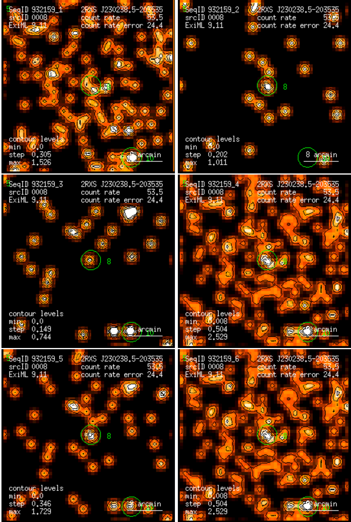
Figure 8: RASS 932159: detection 0008: band rate images, Gaussian filter: (1) PSPC channels 11 – 41, (2) 52 – 90, (3) 91 – 201, (4) 11 – 235, (5) 52 – 201, (6) 11 – 201. Broad band rates in counts/ks. Band rate contour levels in counts/ks/arcmin 2 .
