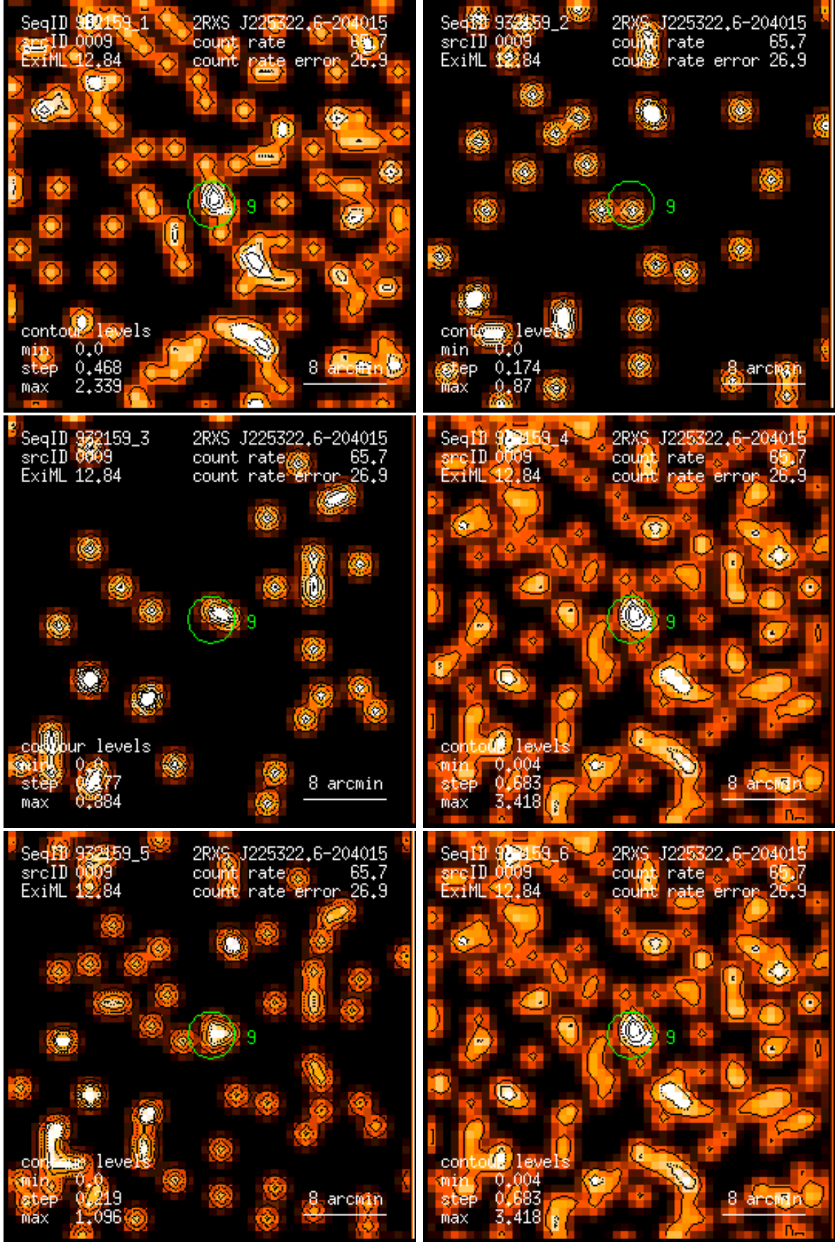
Figure 9: RASS 932159: detection 0009: band rate images, Gaussian filter: (1) PSPC channels 11 – 41, (2) 52 – 90, (3) 91 – 201, (4) 11 – 235, (5) 52 – 201, (6) 11 – 201. Broad band rates in counts/ks. Band rate contour levels in counts/ks/arcmin 2 .
