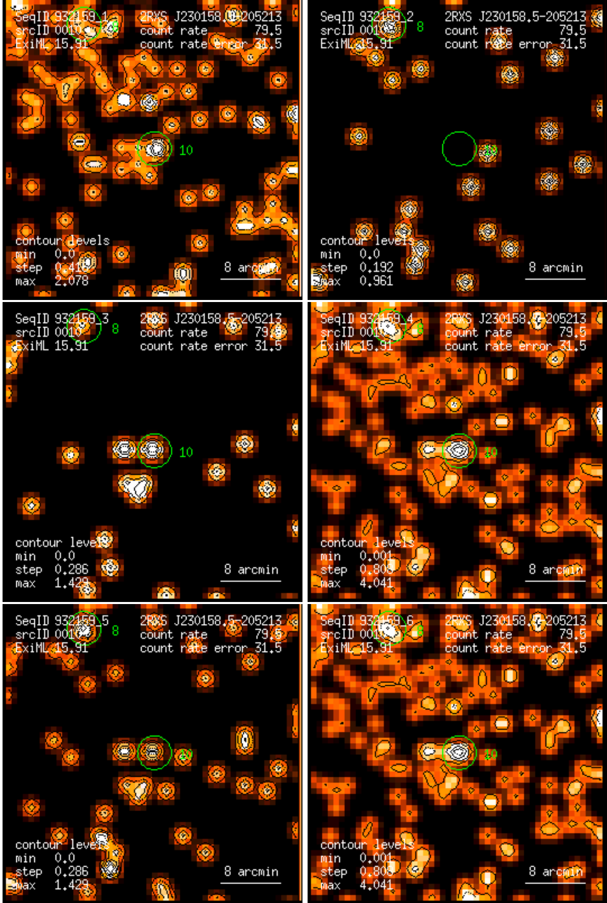
Figure 10: RASS 932159: detection 0010: band rate images, Gaussian filter: (1) PSPC channels 11 – 41, (2) 52 – 90, (3) 91 – 201, (4) 11 – 235, (5) 52 – 201, (6) 11 – 201. Broad band rates in counts/ks. Band rate contour levels in counts/ks/arcmin 2 .
