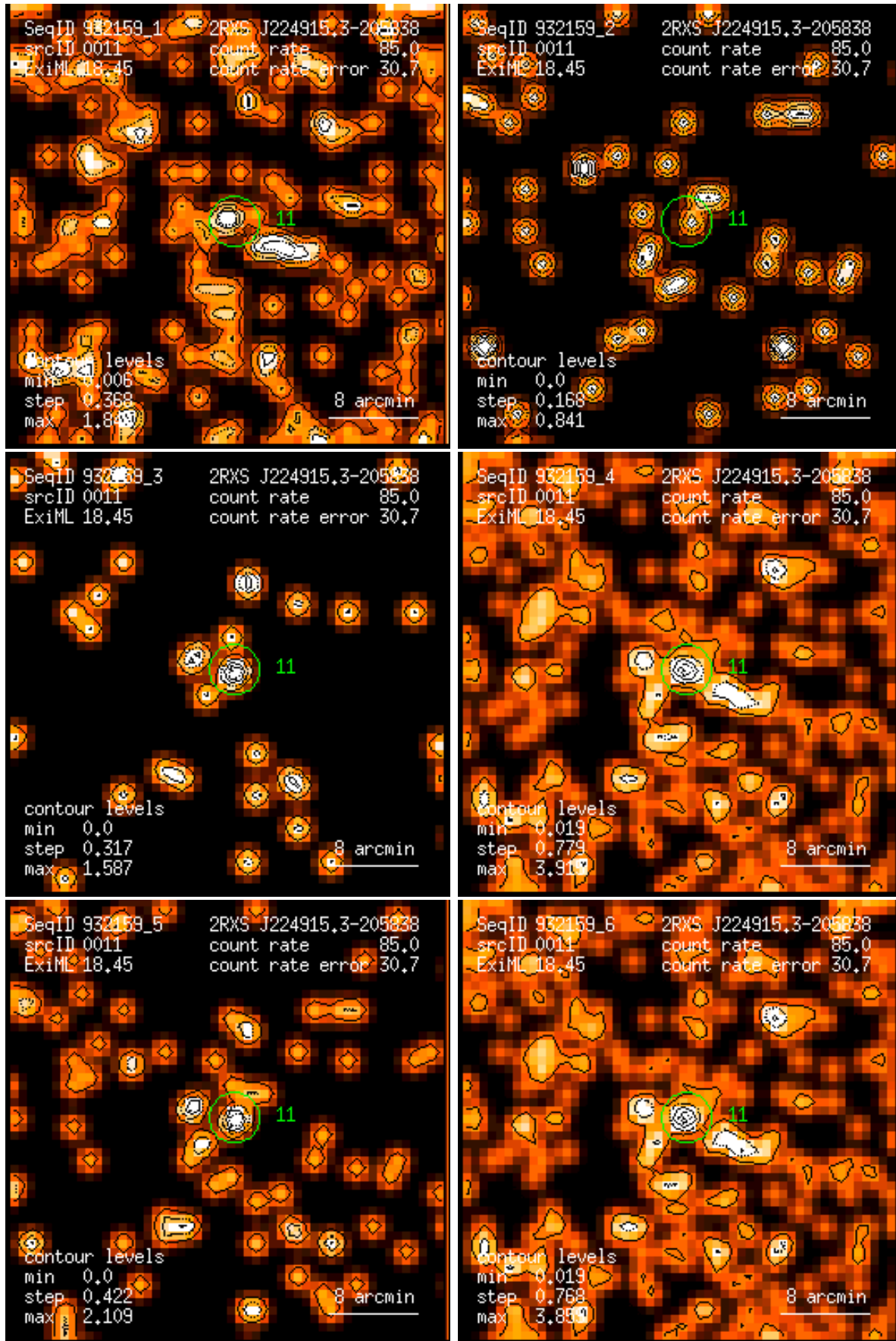
Figure 11: RASS 932159: detection 0011: band rate images, Gaussian filter: (1) PSPC channels 11 – 41, (2) 52 – 90, (3) 91 – 201, (4) 11 – 235, (5) 52 – 201, (6) 11 – 201. Broad band rates in counts/ks. Band rate contour levels in counts/ks/arcmin 2 .
