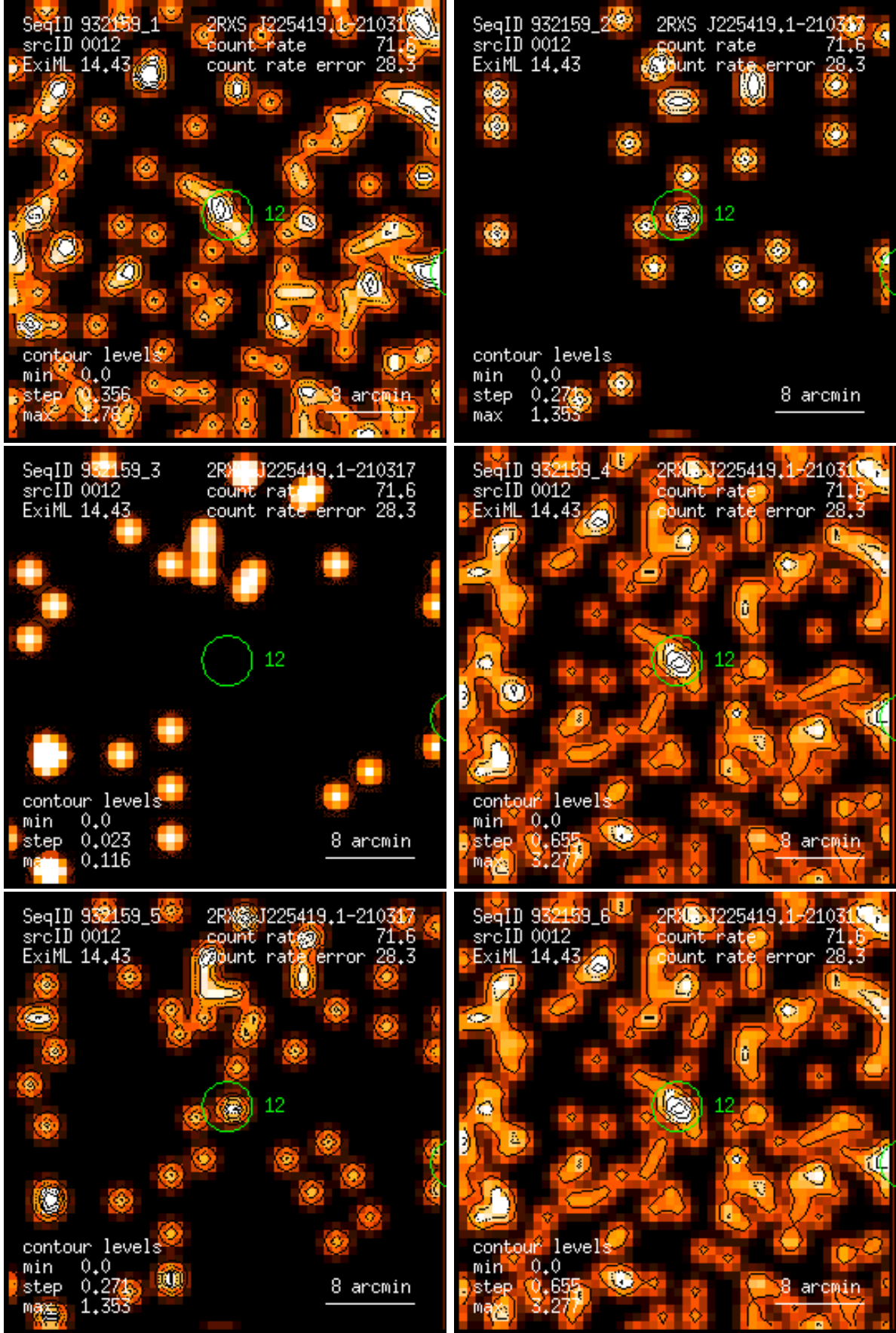
Figure 12: RASS 932159: detection 0012: band rate images, Gaussian filter: (1) PSPC channels 11 – 41, (2) 52 – 90, (3) 91 – 201, (4) 11 – 235, (5) 52 – 201, (6) 11 – 201. Broad band rates in counts/ks. Band rate contour levels in counts/ks/arcmin 2 .
