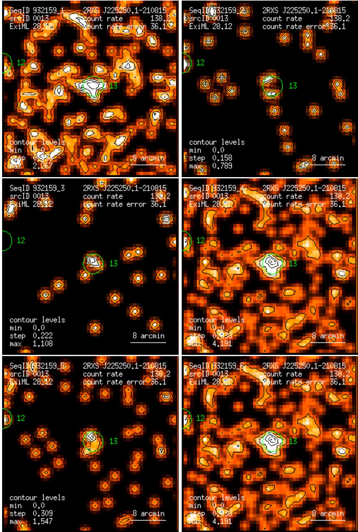
Figure 13: RASS 932159: detection 0013: band rate images, Gaussian filter: (1) PSPC channels 11 – 41, (2) 52 – 90, (3) 91 – 201, (4) 11 – 235, (5) 52 – 201, (6) 11 – 201. Broad band rates in counts/ks. Band rate contour levels in counts/ks/arcmin 2 .
