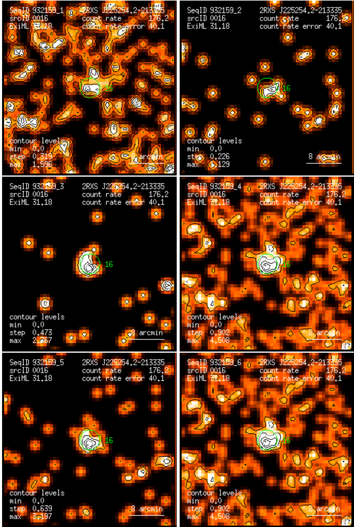
Figure 16: RASS 932159: detection 0016: band rate images, Gaussian filter: (1) PSPC channels 11 – 41, (2) 52 – 90, (3) 91 – 201, (4) 11 – 235, (5) 52 – 201, (6) 11 – 201. Broad band rates in counts/ks. Band rate contour levels in counts/ks/arcmin 2 .
