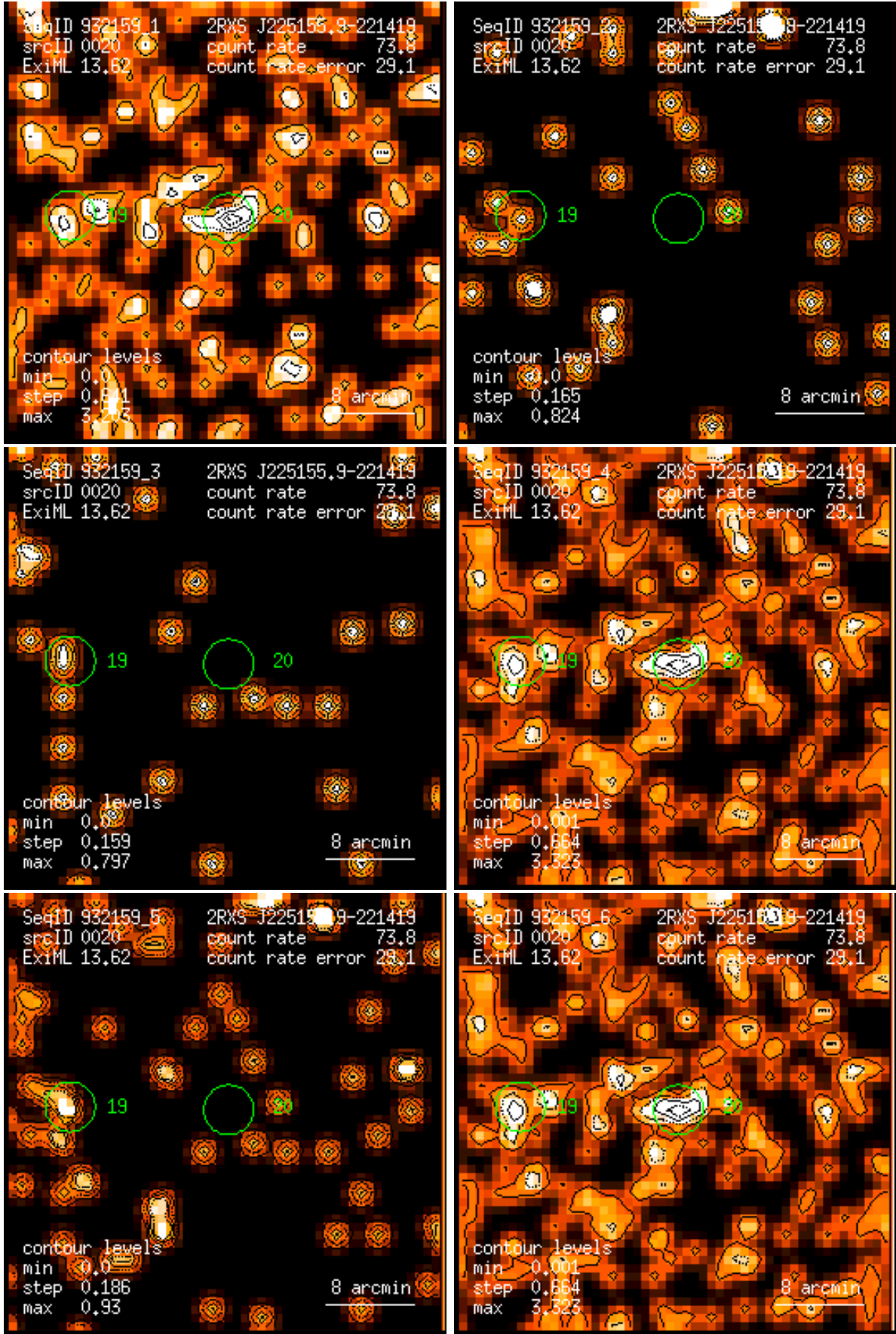
Figure 20: RASS 932159: detection 0020: band rate images, Gaussian filter: (1) PSPC channels 11 – 41, (2) 52 – 90, (3) 91 – 201, (4) 11 – 235, (5) 52 – 201, (6) 11 – 201. Broad band rates in counts/ks. Band rate contour levels in counts/ks/arcmin 2 .
