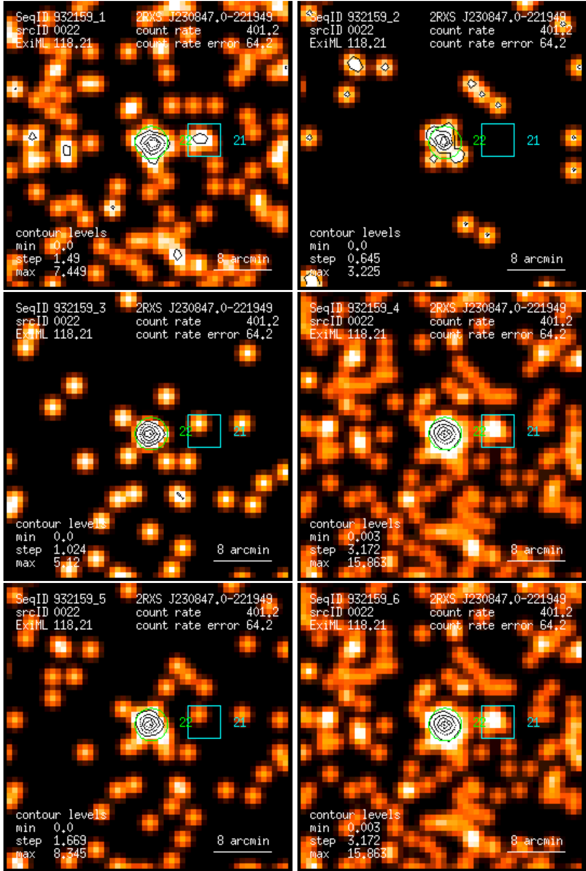
Figure 22: RASS 932159: detection 0022: band rate images, Gaussian filter: (1) PSPC channels 11 – 41, (2) 52 – 90, (3) 91 – 201, (4) 11 – 235, (5) 52 – 201, (6) 11 – 201. Broad band rates in counts/ks. Band rate contour levels in counts/ks/arcmin 2 .
