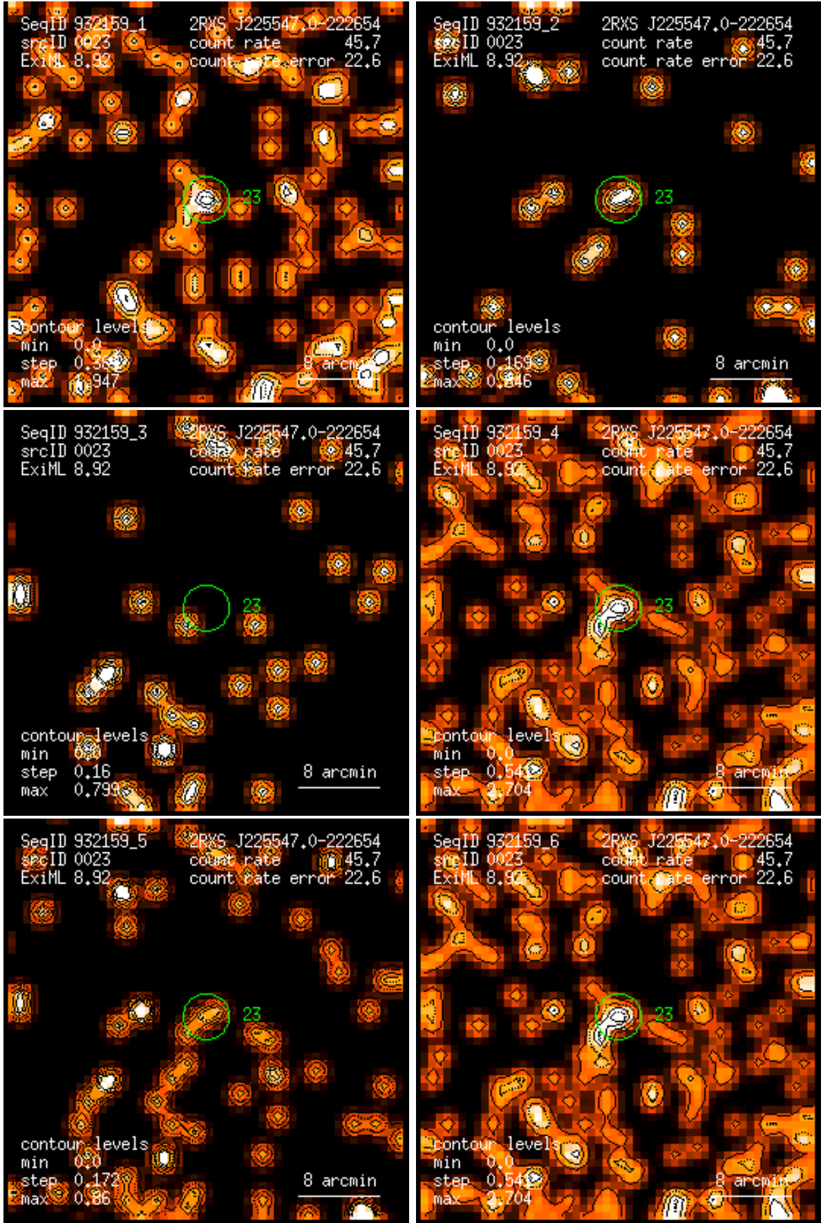
Figure 23: RASS 932159: detection 0023: band rate images, Gaussian filter: (1) PSPC channels 11 – 41, (2) 52 – 90, (3) 91 – 201, (4) 11 – 235, (5) 52 – 201, (6) 11 – 201. Broad band rates in counts/ks. Band rate contour levels in counts/ks/arcmin 2 .
