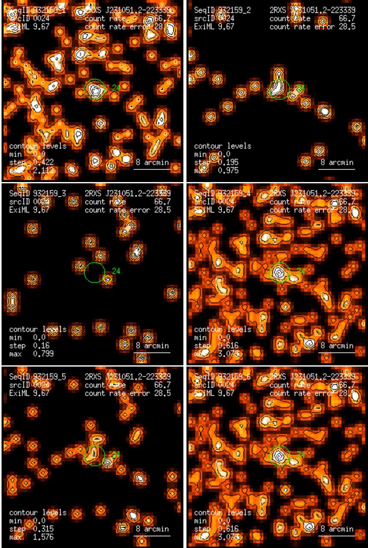
Figure 24: RASS 932159: detection 0024: band rate images, Gaussian filter: (1) PSPC channels 11 – 41, (2) 52 – 90, (3) 91 – 201, (4) 11 – 235, (5) 52 – 201, (6) 11 – 201. Broad band rates in counts/ks. Band rate contour levels in counts/ks/arcmin 2 .
