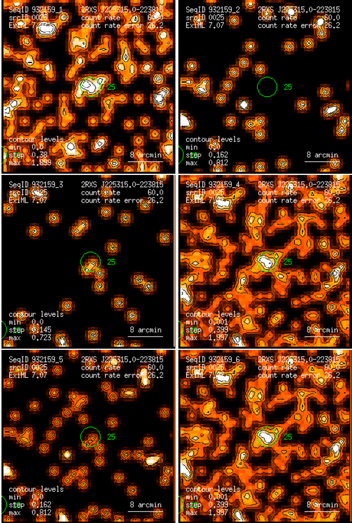
Figure 25: RASS 932159: detection 0025: band rate images, Gaussian filter: (1) PSPC channels 11 – 41, (2) 52 – 90, (3) 91 – 201, (4) 11 – 235, (5) 52 – 201, (6) 11 – 201. Broad band rates in counts/ks. Band rate contour levels in counts/ks/arcmin 2 .
