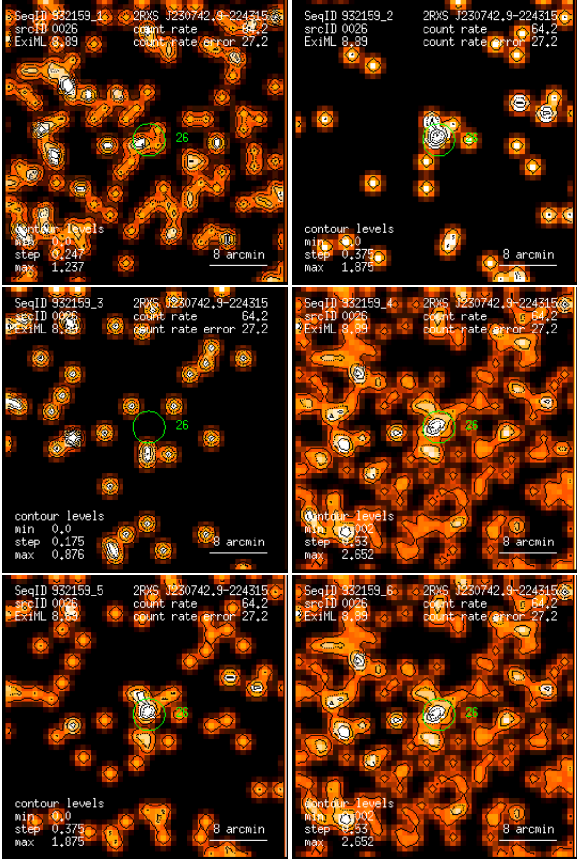
Figure 26: RASS 932159: detection 0026: band rate images, Gaussian filter: (1) PSPC channels 11 – 41, (2) 52 – 90, (3) 91 – 201, (4) 11 – 235, (5) 52 – 201, (6) 11 – 201. Broad band rates in counts/ks. Band rate contour levels in counts/ks/arcmin 2 .
