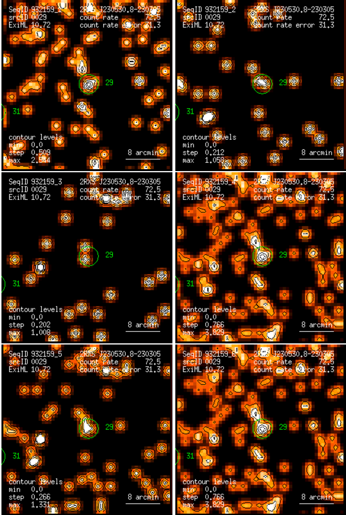
Figure 29: RASS 932159: detection 0029: band rate images, Gaussian filter: (1) PSPC channels 11 – 41, (2) 52 – 90, (3) 91 – 201, (4) 11 – 235, (5) 52 – 201, (6) 11 – 201. Broad band rates in counts/ks. Band rate contour levels in counts/ks/arcmin 2 .
