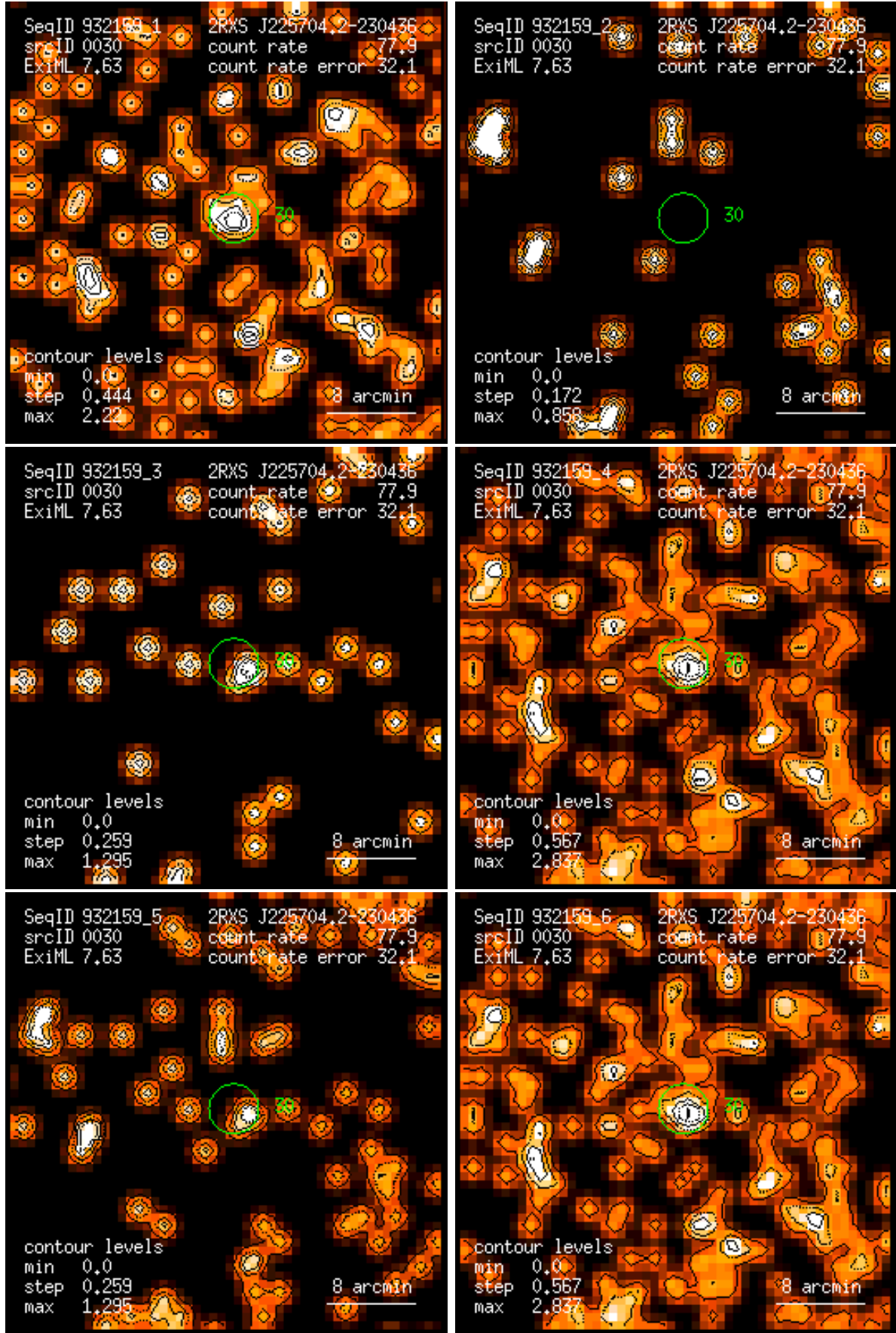
Figure 30: RASS 932159: detection 0030: band rate images, Gaussian filter: (1) PSPC channels 11 – 41, (2) 52 – 90, (3) 91 – 201, (4) 11 – 235, (5) 52 – 201, (6) 11 – 201. Broad band rates in counts/ks. Band rate contour levels in counts/ks/arcmin 2 .
