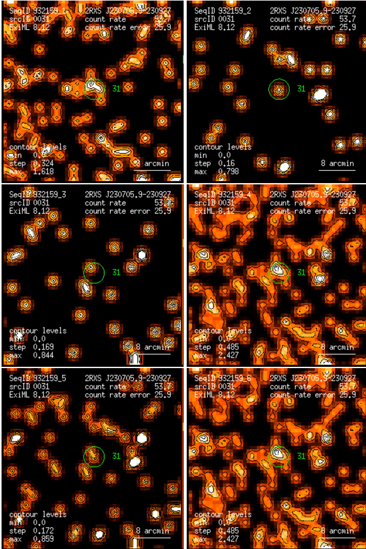
Figure 31: RASS 932159: detection 0031: band rate images, Gaussian filter: (1) PSPC channels 11 – 41, (2) 52 – 90, (3) 91 – 201, (4) 11 – 235, (5) 52 – 201, (6) 11 – 201. Broad band rates in counts/ks. Band rate contour levels in counts/ks/arcmin 2 .
