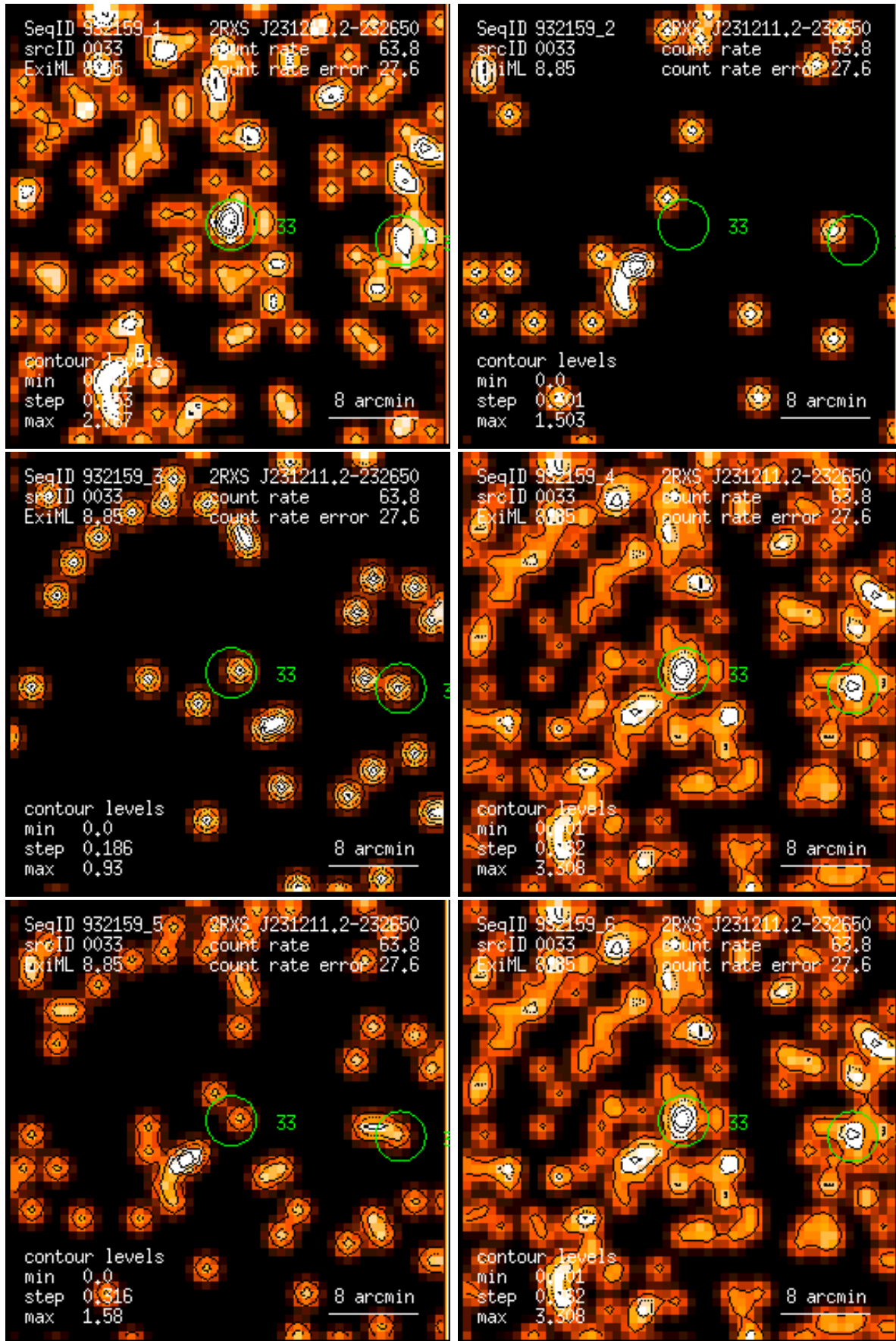
Figure 33: RASS 932159: detection 0033: band rate images, Gaussian filter: (1) PSPC channels 11 – 41, (2) 52 – 90, (3) 91 – 201, (4) 11 – 235, (5) 52 – 201, (6) 11 – 201. Broad band rates in counts/ks. Band rate contour levels in counts/ks/arcmin 2 .
