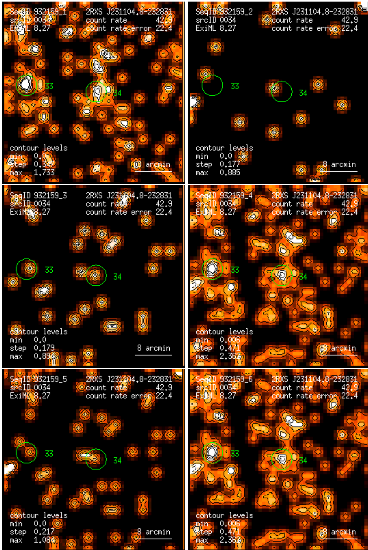
Figure 34: RASS 932159: detection 0034: band rate images, Gaussian filter: (1) PSPC channels 11 – 41, (2) 52 – 90, (3) 91 – 201, (4) 11 – 235, (5) 52 – 201, (6) 11 – 201. Broad band rates in counts/ks. Band rate contour levels in counts/ks/arcmin 2 .
