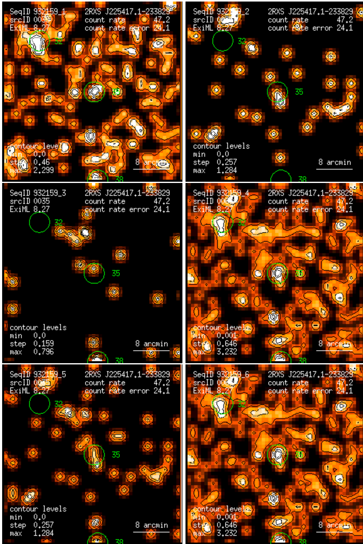
Figure 35: RASS 932159: detection 0035: band rate images, Gaussian filter: (1) PSPC channels 11 – 41, (2) 52 – 90, (3) 91 – 201, (4) 11 – 235, (5) 52 – 201, (6) 11 – 201. Broad band rates in counts/ks. Band rate contour levels in counts/ks/arcmin 2 .
