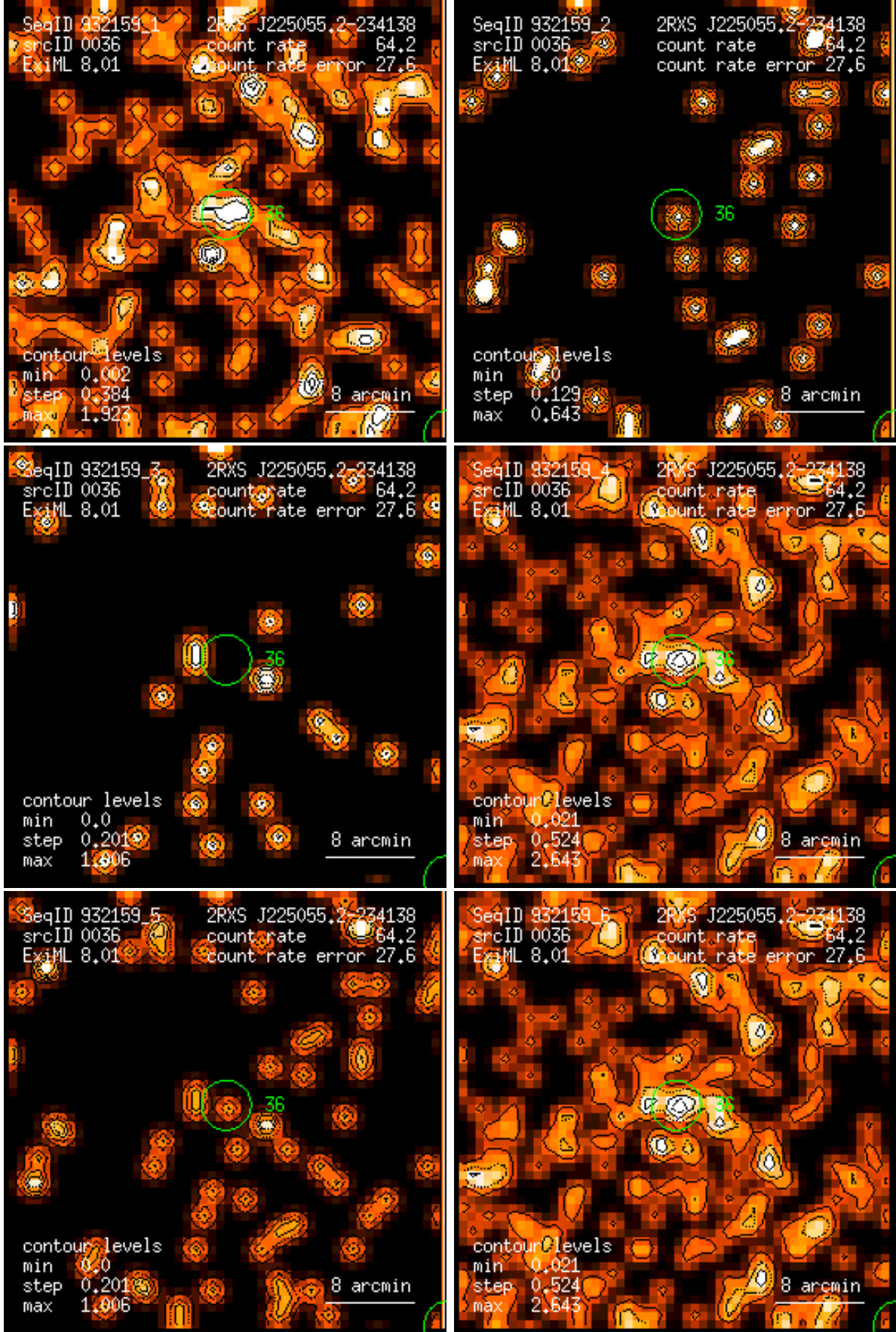
Figure 36: RASS 932159: detection 0036: band rate images, Gaussian filter: (1) PSPC channels 11 – 41, (2) 52 – 90, (3) 91 – 201, (4) 11 – 235, (5) 52 – 201, (6) 11 – 201. Broad band rates in counts/ks. Band rate contour levels in counts/ks/arcmin 2 .
