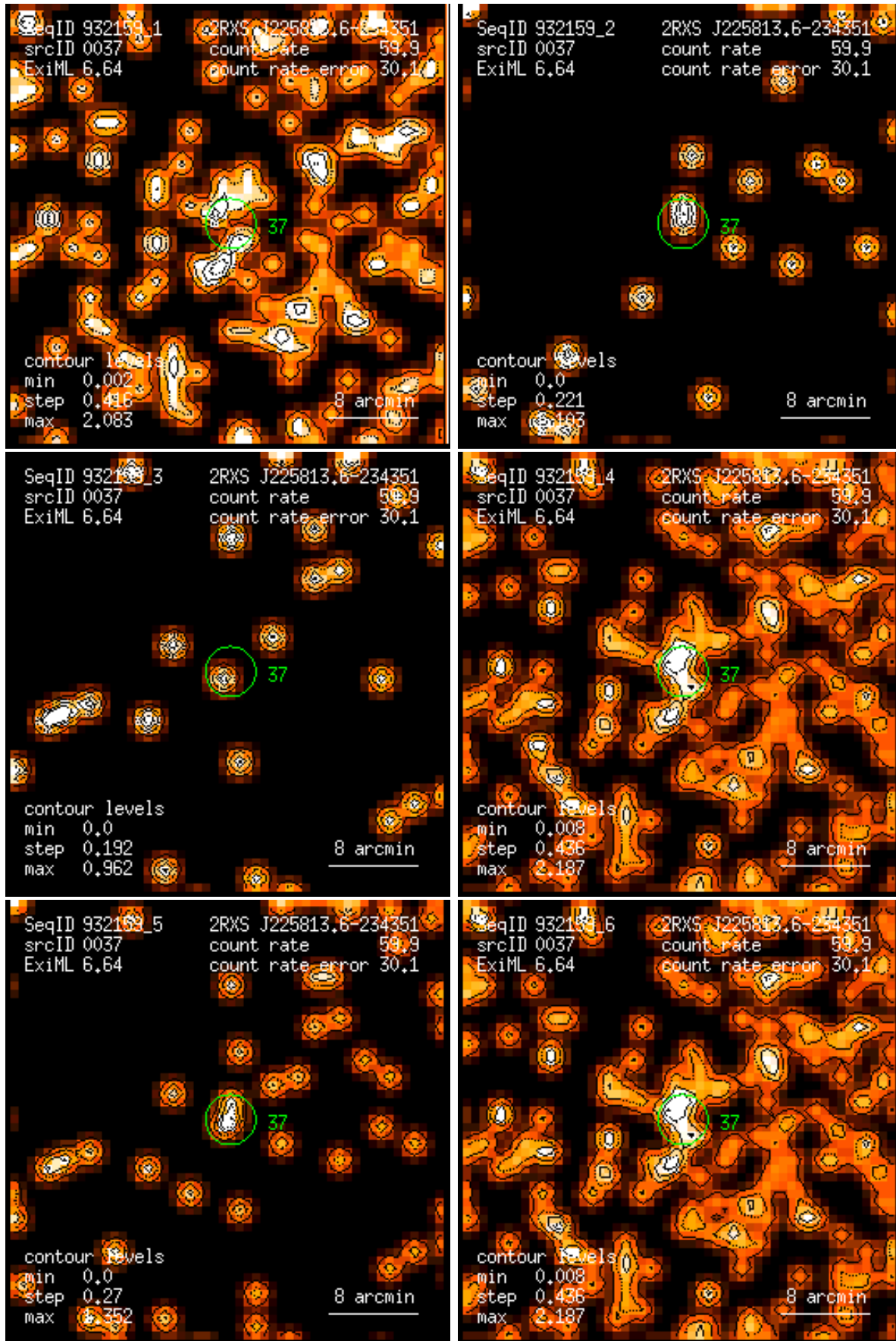
Figure 37: RASS 932159: detection 0037: band rate images, Gaussian filter: (1) PSPC channels 11 – 41, (2) 52 – 90, (3) 91 – 201, (4) 11 – 235, (5) 52 – 201, (6) 11 – 201. Broad band rates in counts/ks. Band rate contour levels in counts/ks/arcmin 2 .
