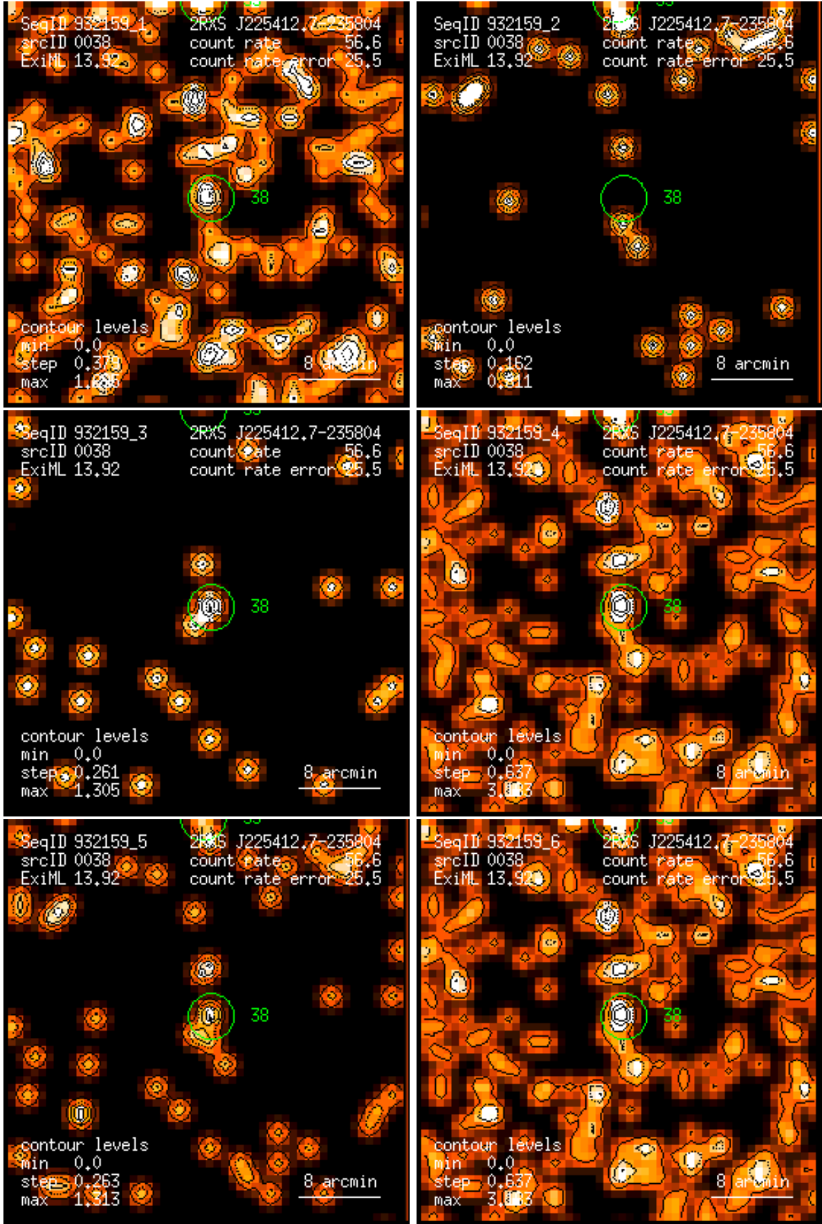
Figure 38: RASS 932159: detection 0038: band rate images, Gaussian filter: (1) PSPC channels 11 – 41, (2) 52 – 90, (3) 91 – 201, (4) 11 – 235, (5) 52 – 201, (6) 11 – 201. Broad band rates in counts/ks. Band rate contour levels in counts/ks/arcmin 2 .
