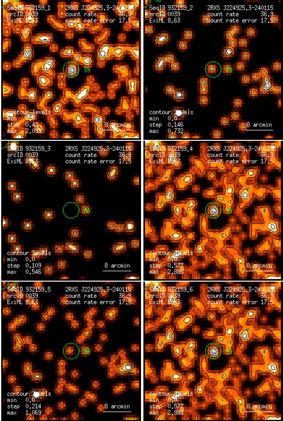
Figure 39: RASS 932159: detection 0039: band rate images, Gaussian filter: (1) PSPC channels 11 – 41, (2) 52 – 90, (3) 91 – 201, (4) 11 – 235, (5) 52 – 201, (6) 11 – 201. Broad band rates in counts/ks. Band rate contour levels in counts/ks/arcmin 2 .
