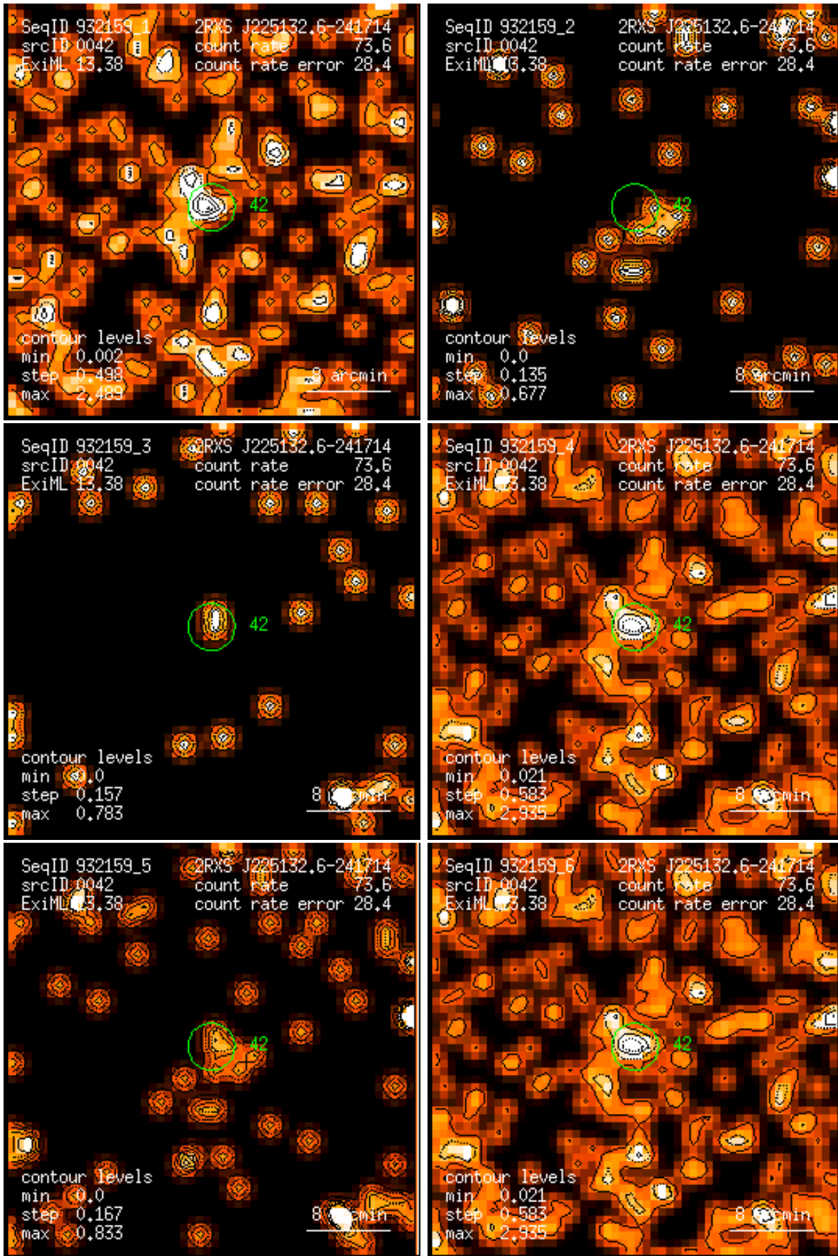
Figure 42: RASS 932159: detection 0042: band rate images, Gaussian filter: (1) PSPC channels 11 – 41, (2) 52 – 90, (3) 91 – 201, (4) 11 – 235, (5) 52 – 201, (6) 11 – 201. Broad band rates in counts/ks. Band rate contour levels in counts/ks/arcmin 2 .
