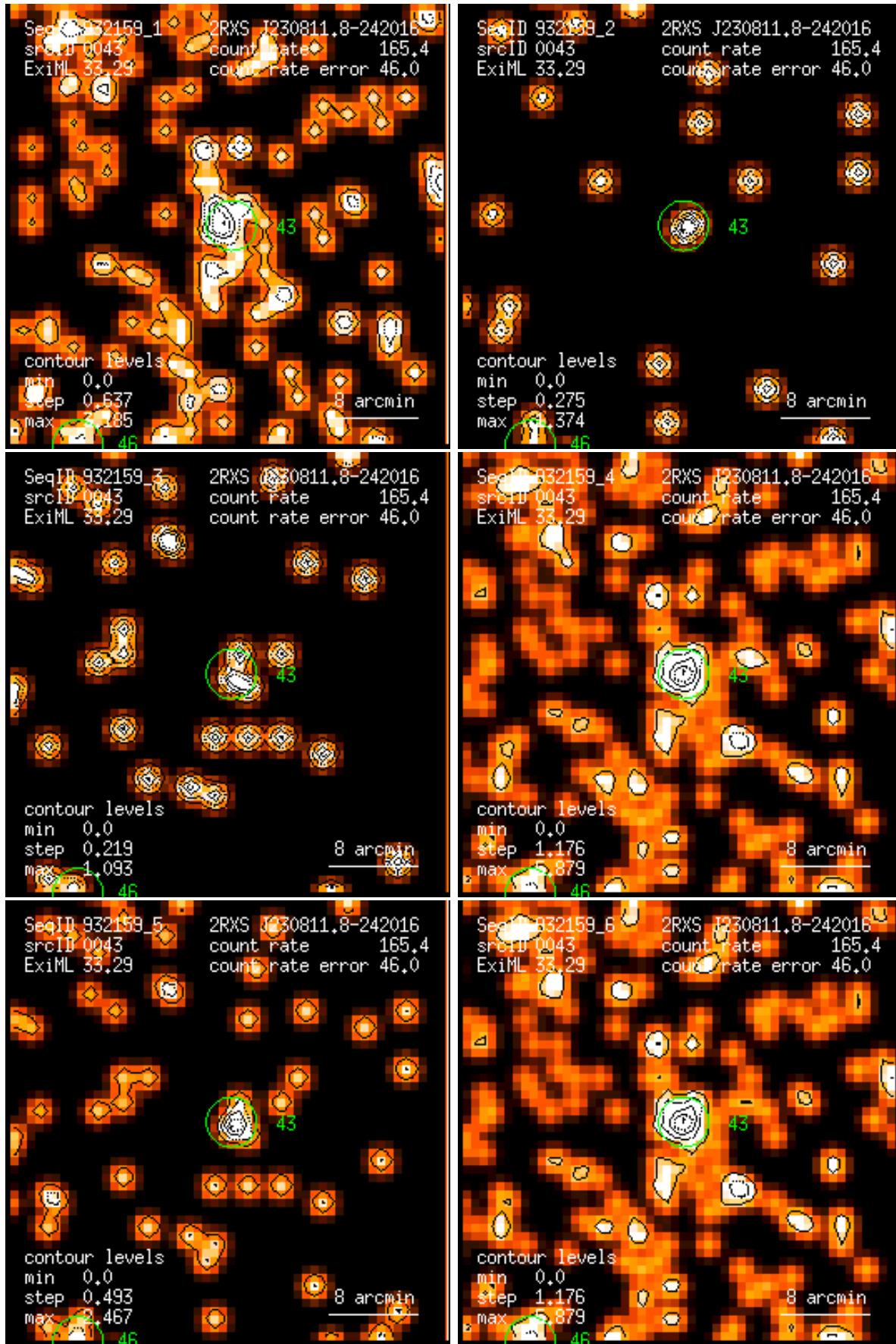
Figure 43: RASS 932159: detection 0043: band rate images, Gaussian filter: (1) PSPC channels 11 – 41, (2) 52 – 90, (3) 91 – 201, (4) 11 – 235, (5) 52 – 201, (6) 11 – 201. Broad band rates in counts/ks. Band rate contour levels in counts/ks/arcmin 2 .
