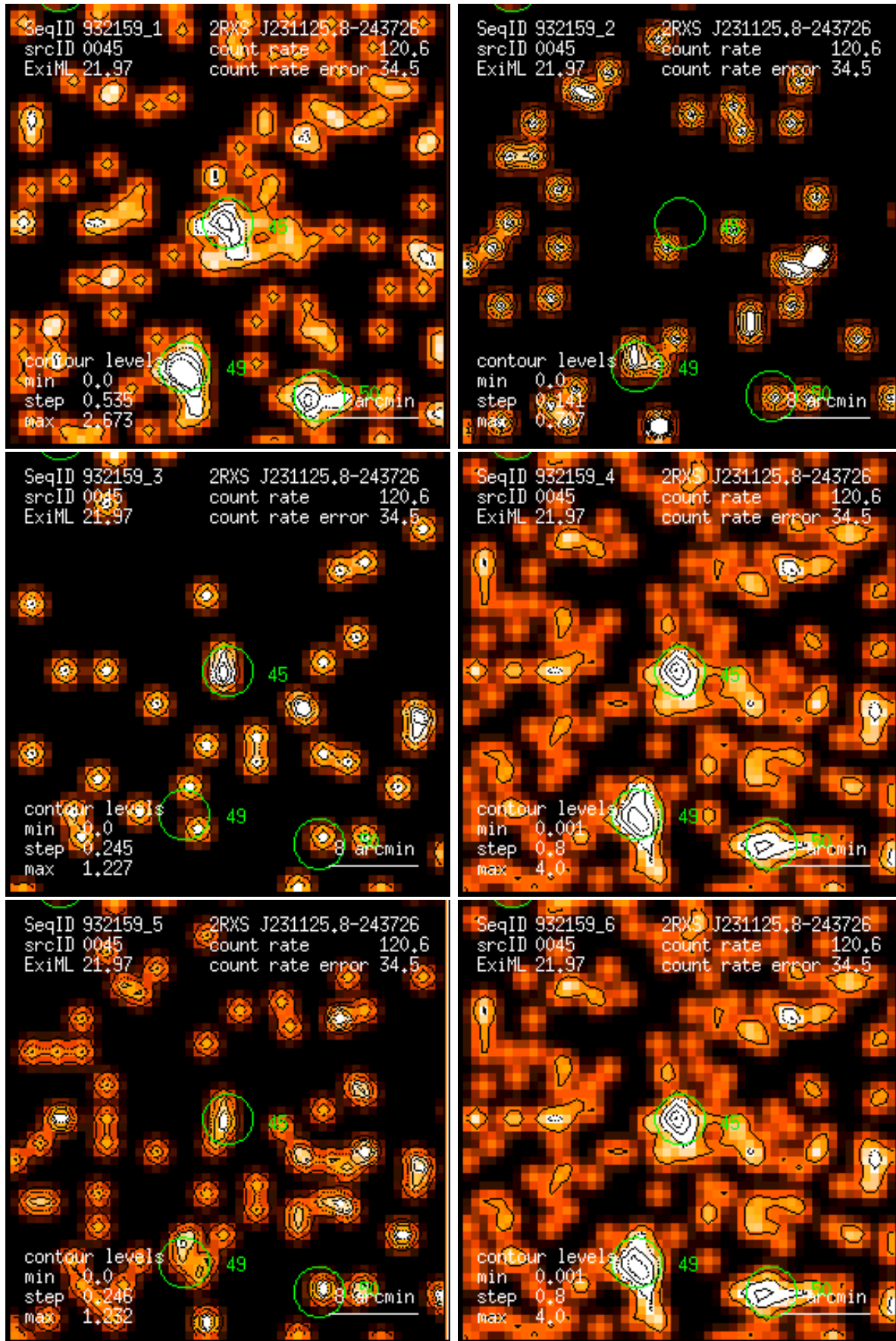
Figure 45: RASS 932159: detection 0045: band rate images, Gaussian filter: (1) PSPC channels 11 – 41, (2) 52 – 90, (3) 91 – 201, (4) 11 – 235, (5) 52 – 201, (6) 11 – 201. Broad band rates in counts/ks. Band rate contour levels in counts/ks/arcmin 2 .
