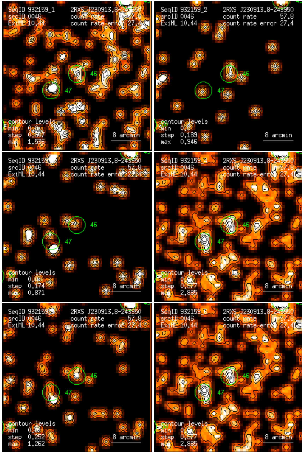
Figure 46: RASS 932159: detection 0046: band rate images, Gaussian filter: (1) PSPC channels 11 – 41, (2) 52 – 90, (3) 91 – 201, (4) 11 – 235, (5) 52 – 201, (6) 11 – 201. Broad band rates in counts/ks. Band rate contour levels in counts/ks/arcmin 2 .
