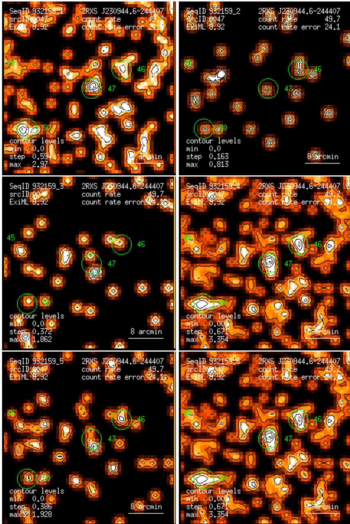
Figure 47: RASS 932159: detection 0047: band rate images, Gaussian filter: (1) PSPC channels 11 – 41, (2) 52 – 90, (3) 91 – 201, (4) 11 – 235, (5) 52 – 201, (6) 11 – 201. Broad band rates in counts/ks. Band rate contour levels in counts/ks/arcmin 2 .
