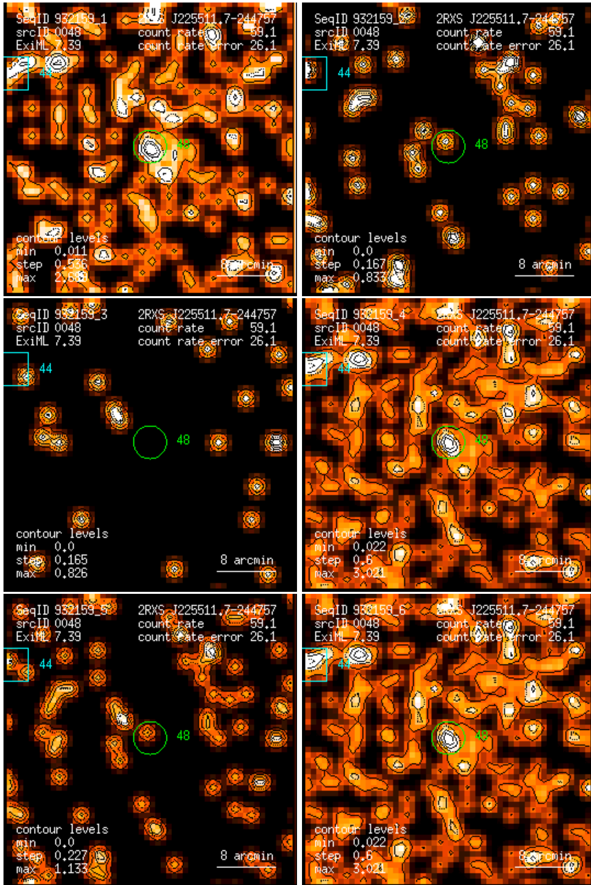
Figure 48: RASS 932159: detection 0048: band rate images, Gaussian filter: (1) PSPC channels 11 – 41, (2) 52 – 90, (3) 91 – 201, (4) 11 – 235, (5) 52 – 201, (6) 11 – 201. Broad band rates in counts/ks. Band rate contour levels in counts/ks/arcmin 2 .
