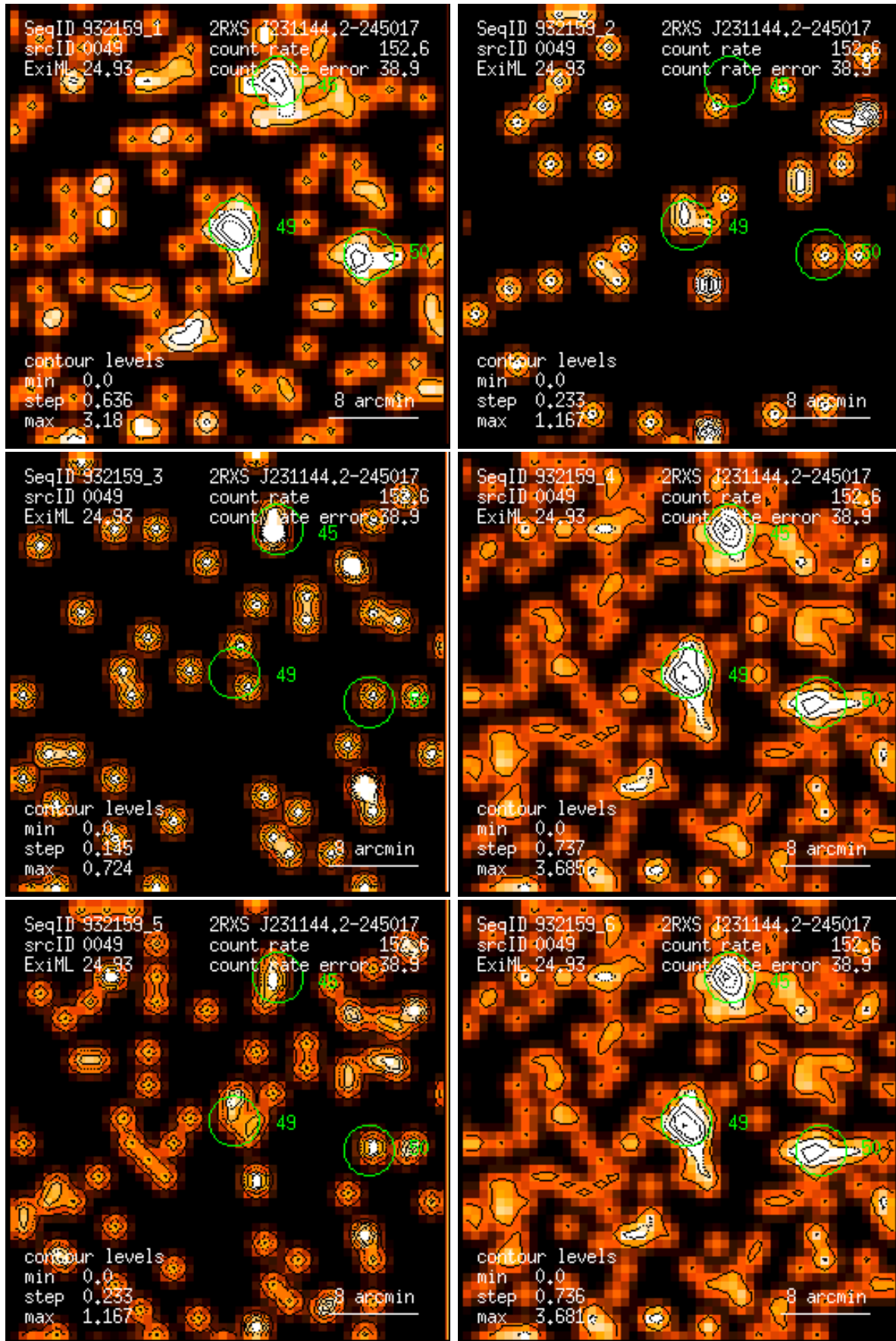
Figure 49: RASS 932159: detection 0049: band rate images, Gaussian filter: (1) PSPC channels 11 – 41, (2) 52 – 90, (3) 91 – 201, (4) 11 – 235, (5) 52 – 201, (6) 11 – 201. Broad band rates in counts/ks. Band rate contour levels in counts/ks/arcmin 2 .
