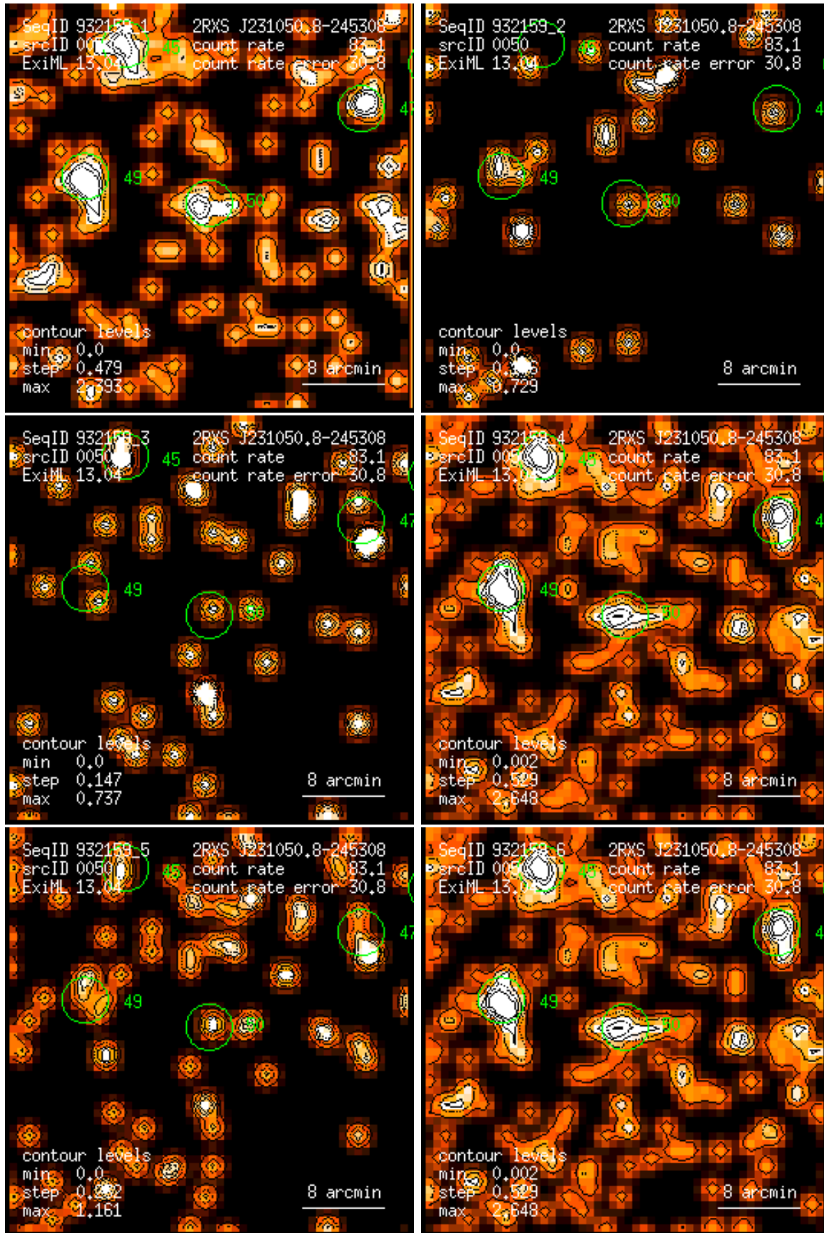
Figure 50: RASS 932159: detection 0050: band rate images, Gaussian filter: (1) PSPC channels 11 – 41, (2) 52 – 90, (3) 91 – 201, (4) 11 – 235, (5) 52 – 201, (6) 11 – 201. Broad band rates in counts/ks. Band rate contour levels in counts/ks/arcmin 2 .
