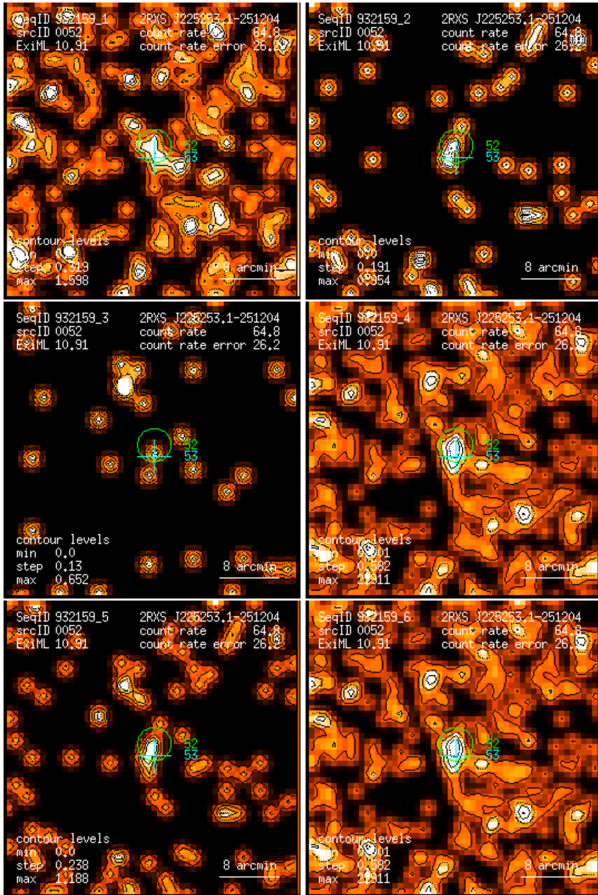
Figure 52: RASS 932159: detection 0052: band rate images, Gaussian filter: (1) PSPC channels 11 – 41, (2) 52 – 90, (3) 91 – 201, (4) 11 – 235, (5) 52 – 201, (6) 11 – 201. Broad band rates in counts/ks. Band rate contour levels in counts/ks/arcmin 2 .
