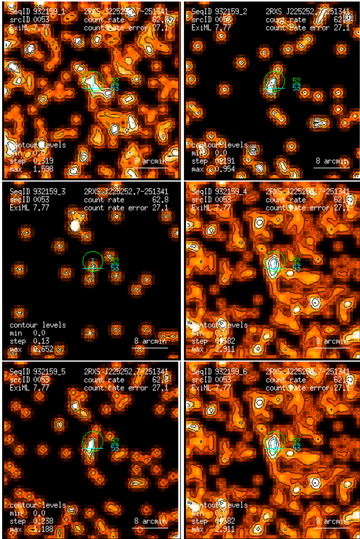
Figure 53: RASS 932159: detection 0053: band rate images, Gaussian filter: (1) PSPC channels 11 – 41, (2) 52 – 90, (3) 91 – 201, (4) 11 – 235, (5) 52 – 201, (6) 11 – 201. Broad band rates in counts/ks. Band rate contour levels in counts/ks/arcmin 2 .
