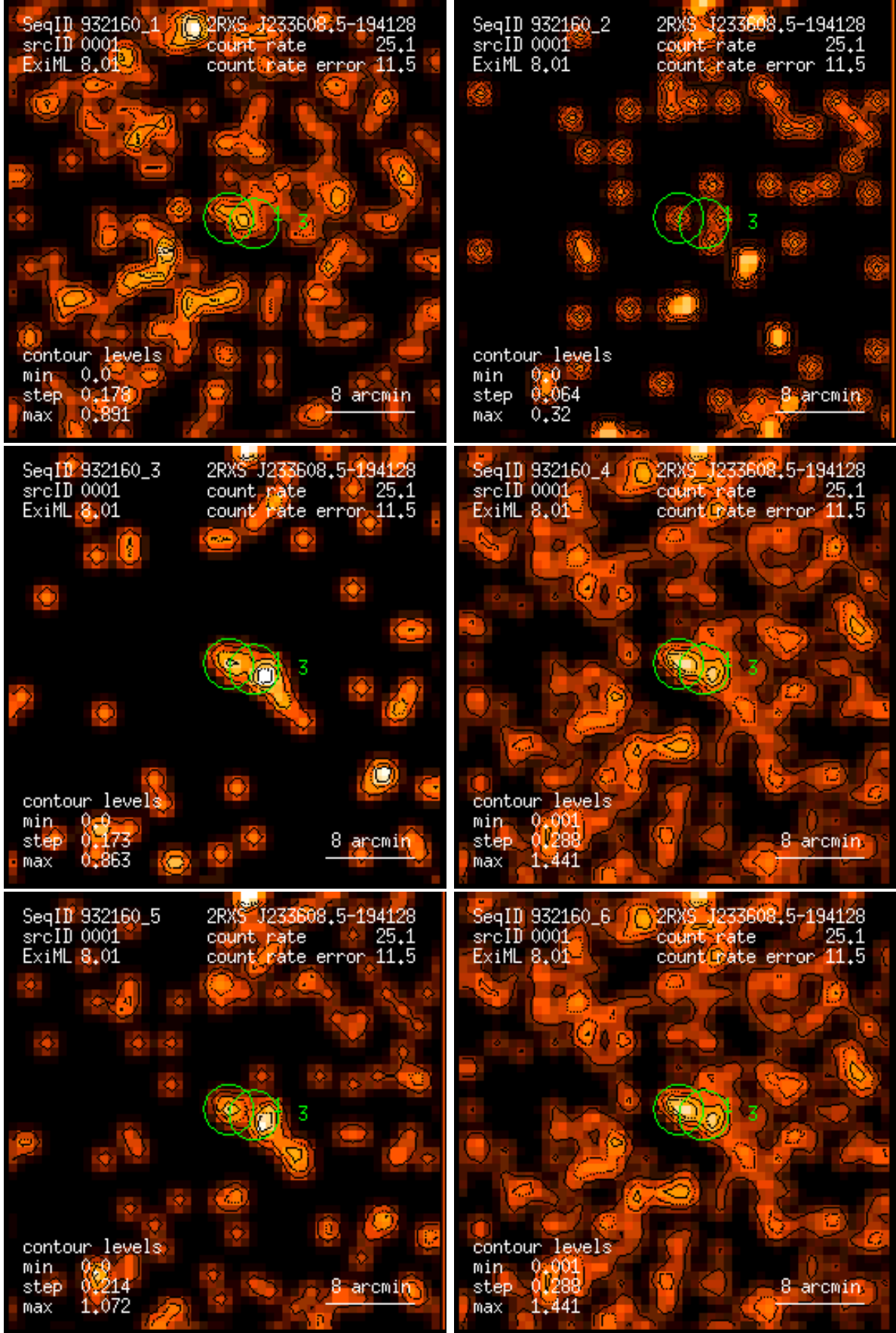
Figure 1: RASS 932160: detection 0001: band rate images, Gaussian filter: (1) PSPC channels 11 – 41, (2) 52 – 90, (3) 91 – 201, (4) 11 – 235, (5) 52 – 201, (6) 11 – 201. Broad band rates in counts/ks. Band rate contour levels in counts/ks/arcmin 2 .
