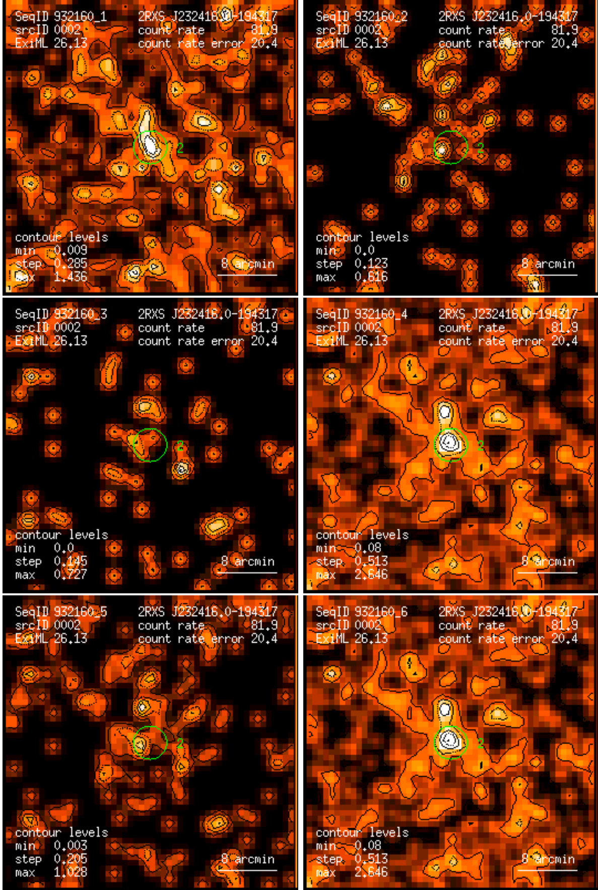
Figure 2: RASS 932160: detection 0002: band rate images, Gaussian filter: (1) PSPC channels 11 – 41, (2) 52 – 90, (3) 91 – 201, (4) 11 – 235, (5) 52 – 201, (6) 11 – 201. Broad band rates in counts/ks. Band rate contour levels in counts/ks/arcmin 2 .
